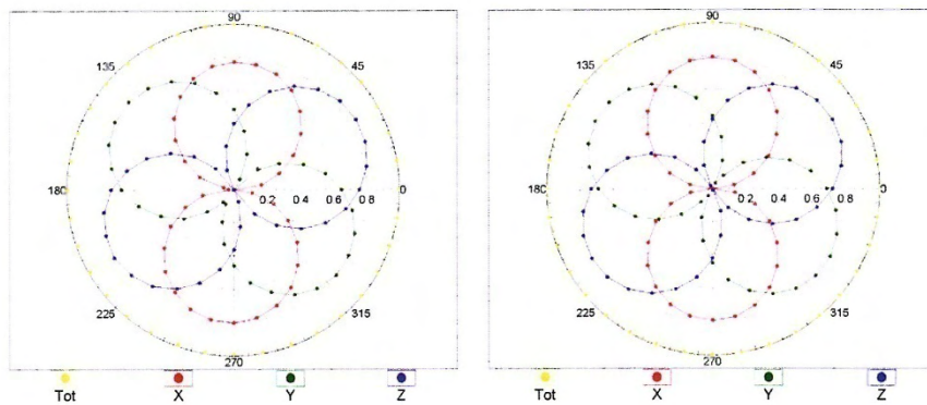
f=600 MHz,TEM
