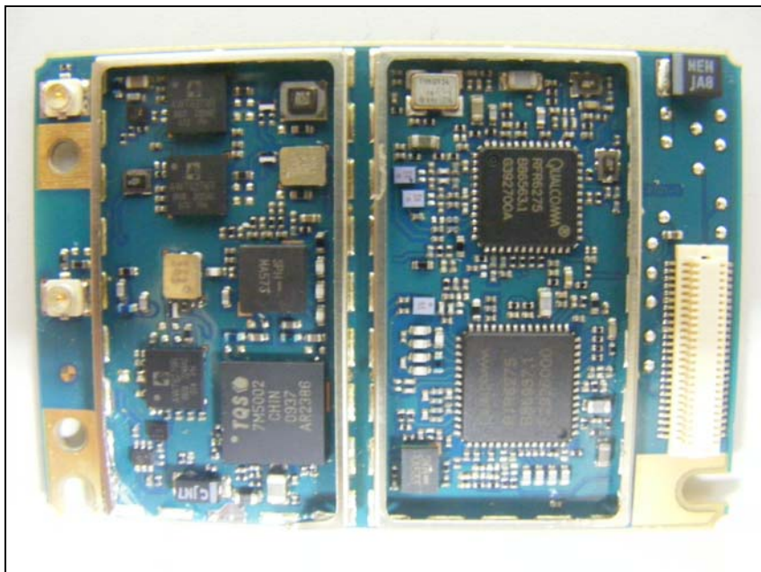
Bottom view of RF module
