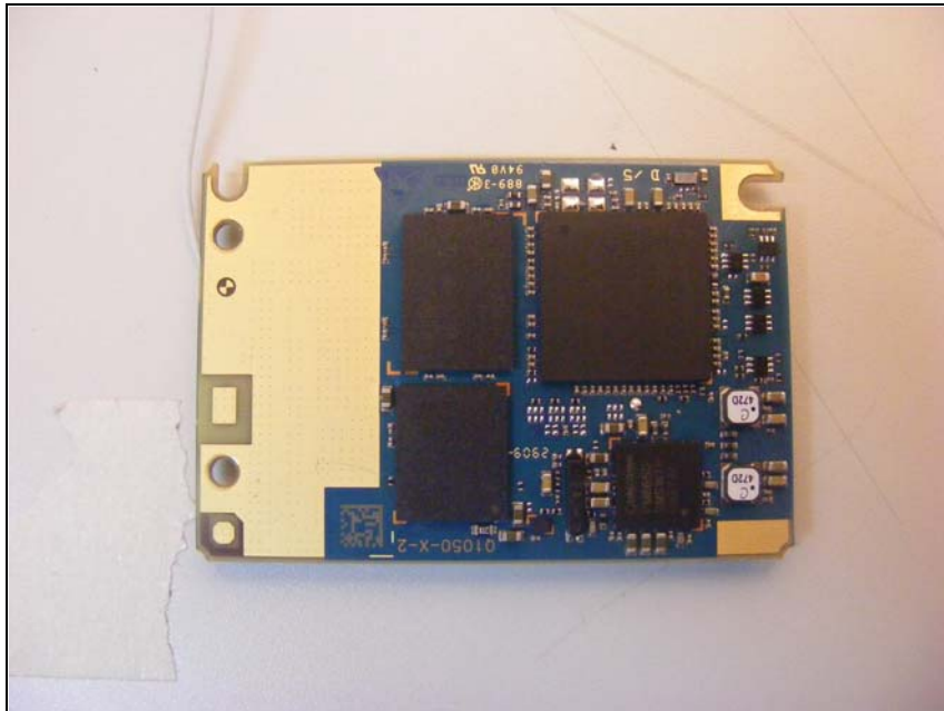
Top view of RF module
