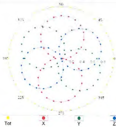
f=600 MHz,TEM
