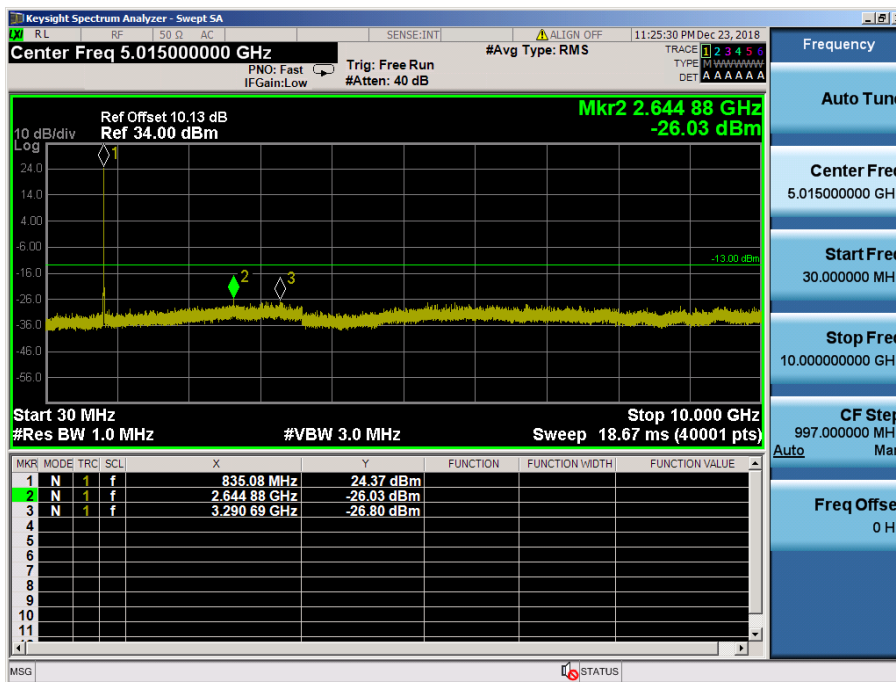
LTE Band 5 / 10MHz / 16QAM - RB Size/Offset (25/12) – Mid Channel
