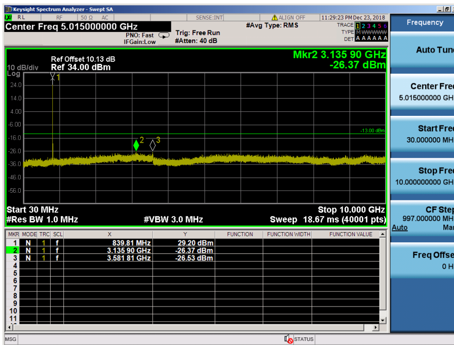
LTE Band 5 / 10MHz / 16QAM - RB Size/Offset (1/0) – High Channel
