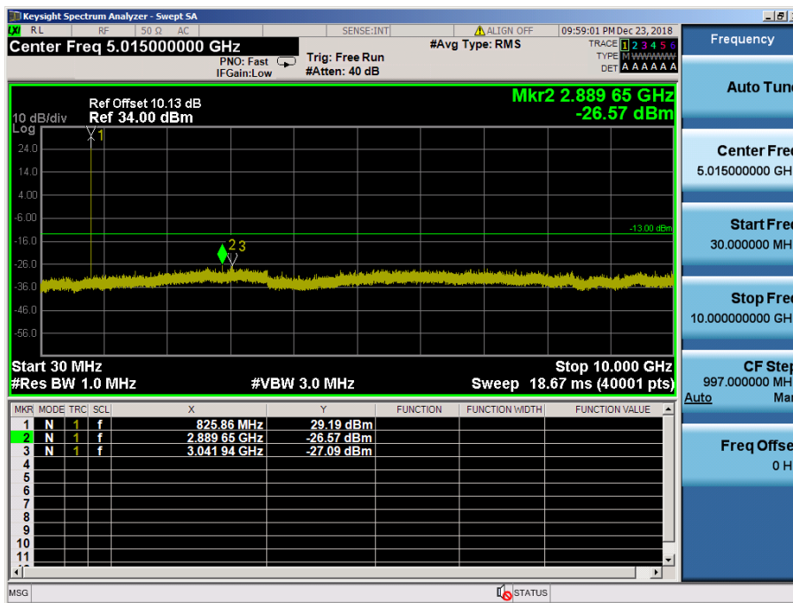
LTE Band 5 / 3MHz / 16QAM - RB Size/Offset (1/7) – Low Channel
