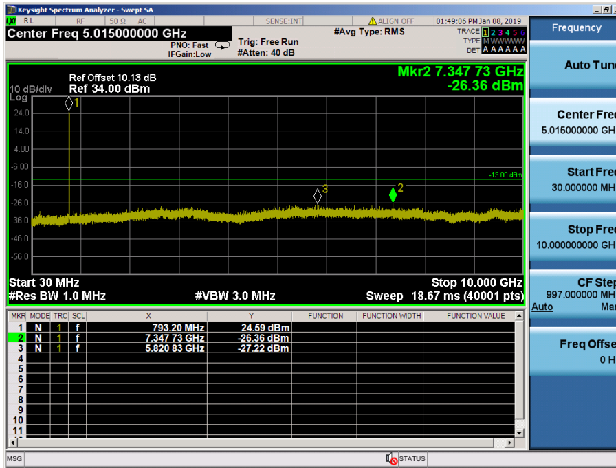
LTE Band 14 / 10MHz / QPSK - RB Size/Offset (25/12) – Low Channel
