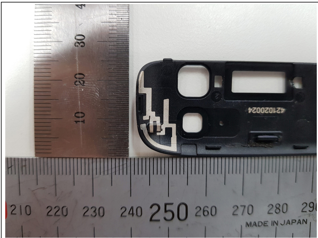
<Option Antenna – Not connected to PCB>
