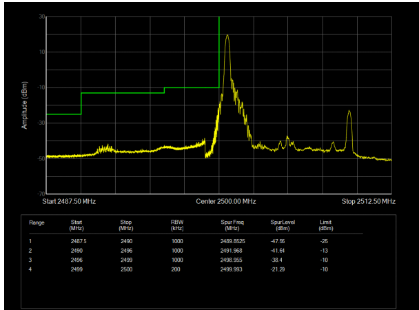
LTE Band 7 64QAM 10MHz CH-Low, 100%RB
