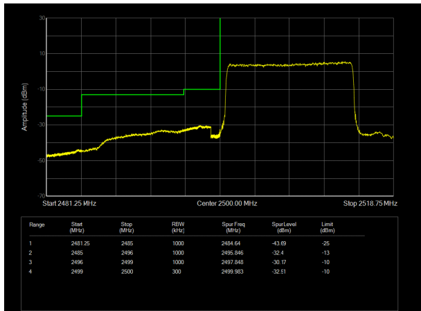
LTE Band 7 QPSK 15MHz CH-Low, 100%RB
