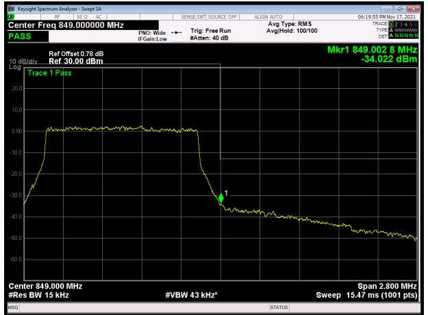
LTE Band 26 64QAM 3MHz CH-High 1RB
