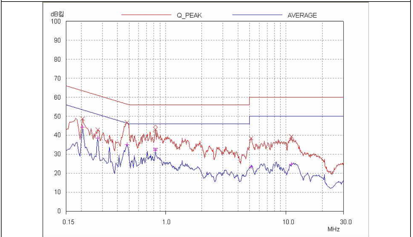
NEUTRAL LINE
