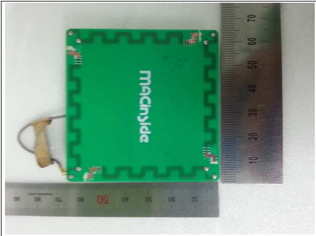
Minimum test separation distance for calculating SAR test exclusion threshold level
