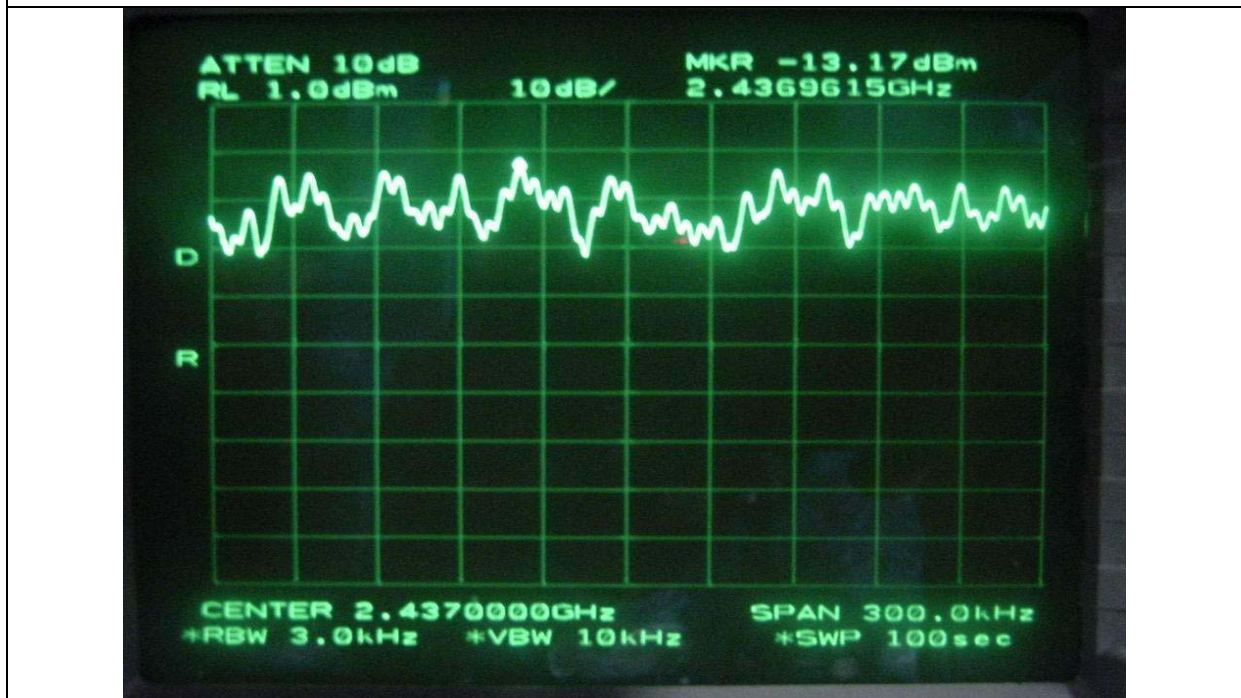
Middle Channel
