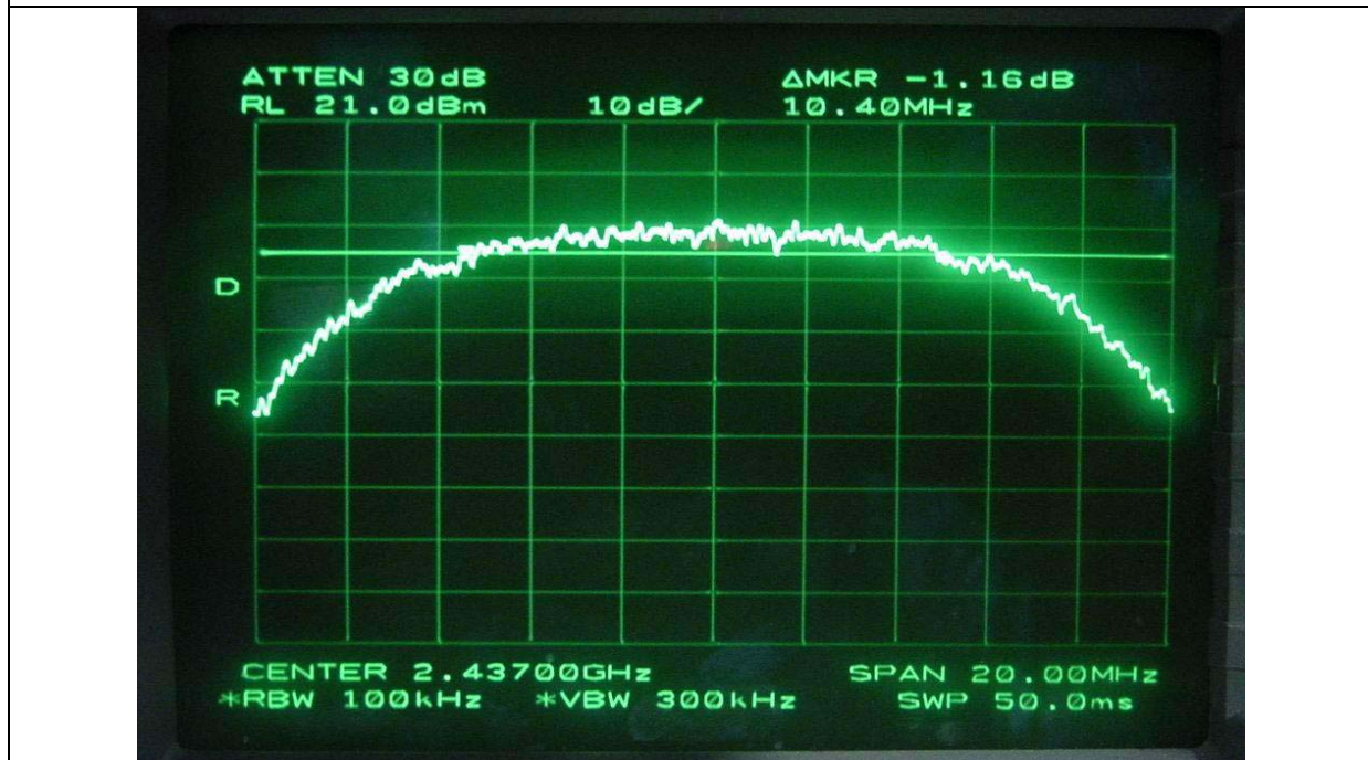
Middle Channel
