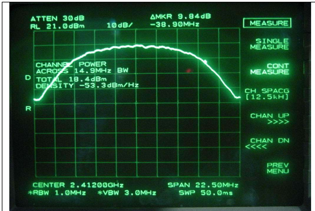
Low Channel
