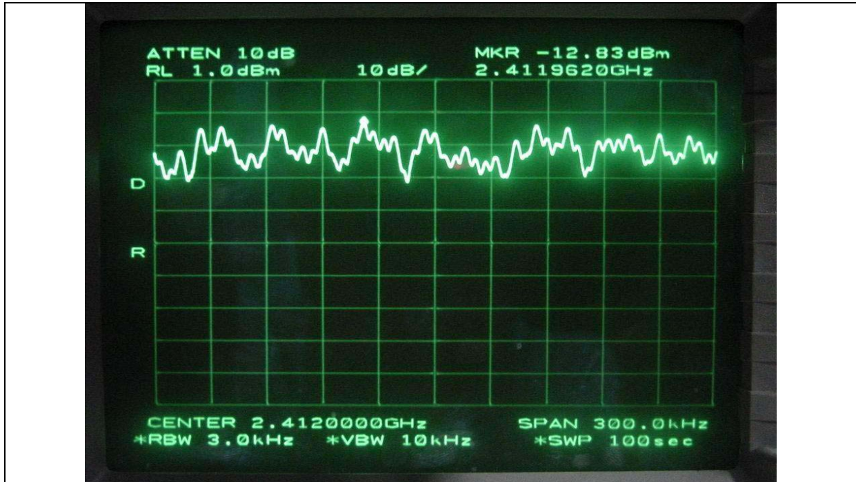
Low Channel
