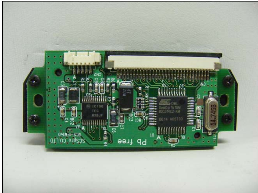
Bottom view of card reader
