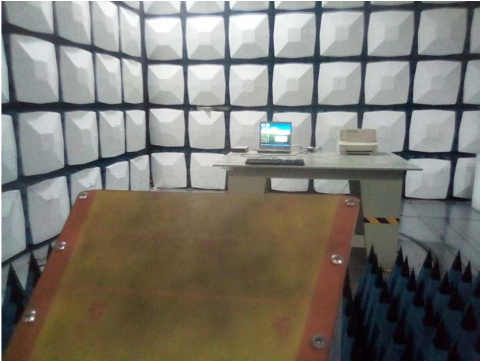
Radiated Emission Above 1GHz – Front View
