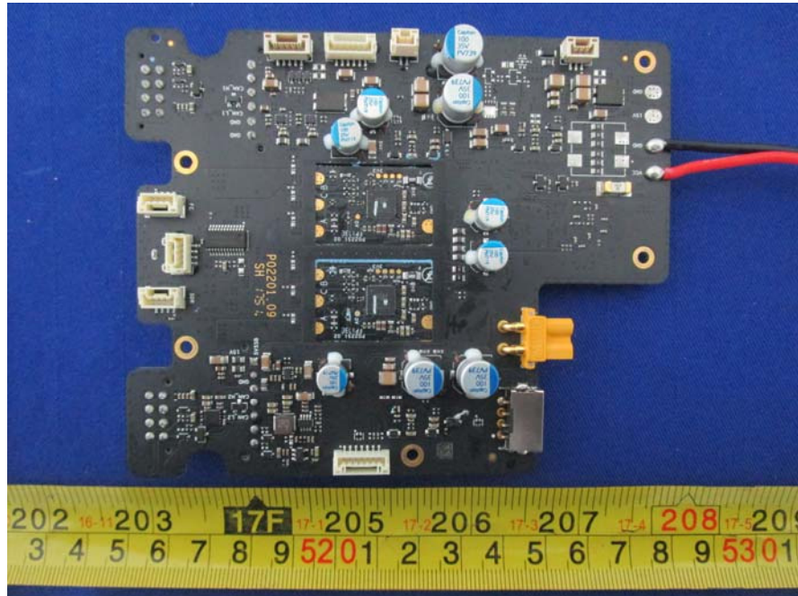
EUT – Center Board Top View
