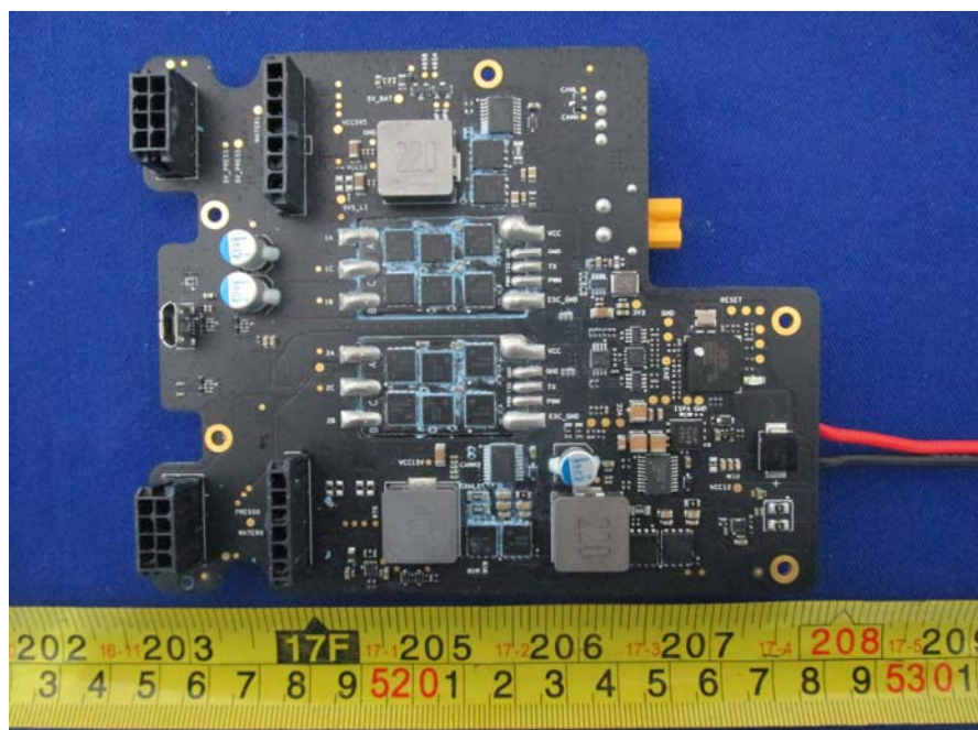
EUT – Center Board Bottom View
