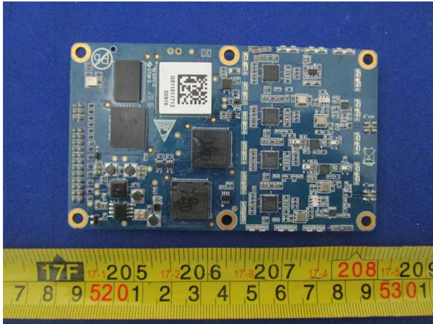
EUT – RTK Module Board Top Uncover View
