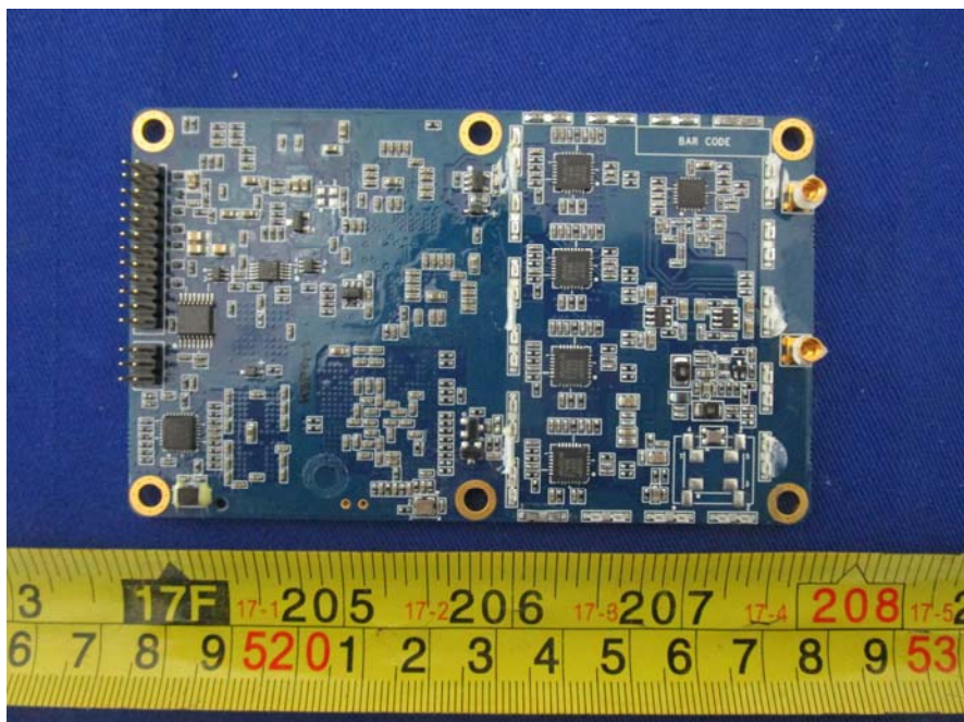
EUT – RTK Module Board Bottom Uncover View
