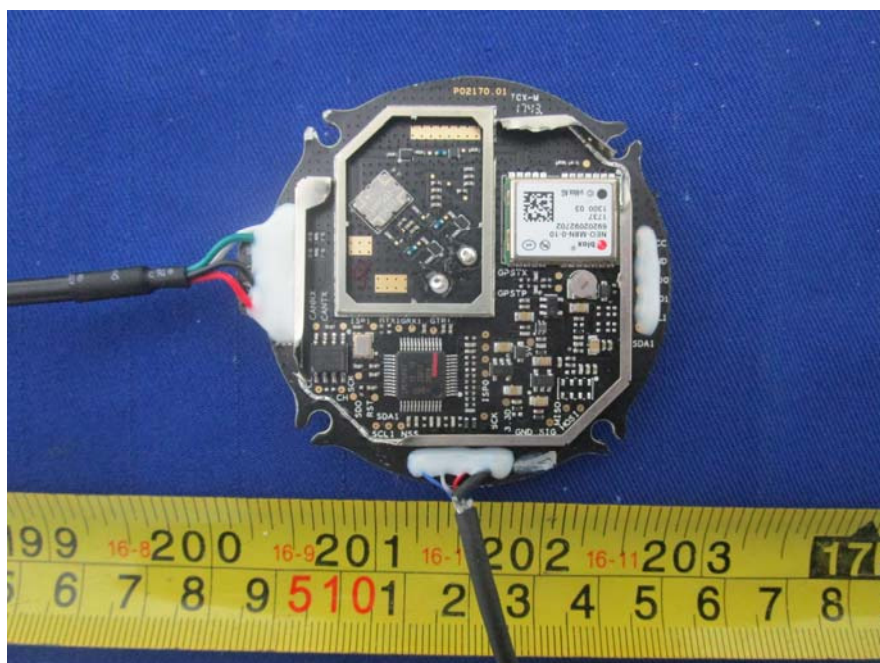
EUT – GPS Module Top Uncover View
