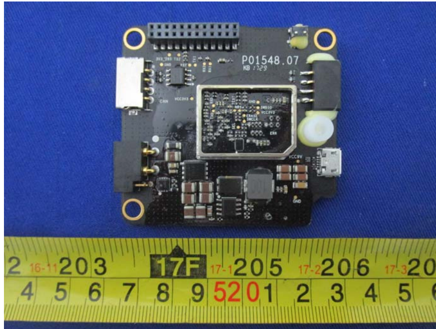
EUT – PCB-3 Top Uncover View
