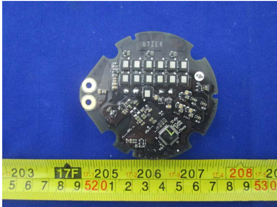
EUT – Motor Control Board Bottom View
