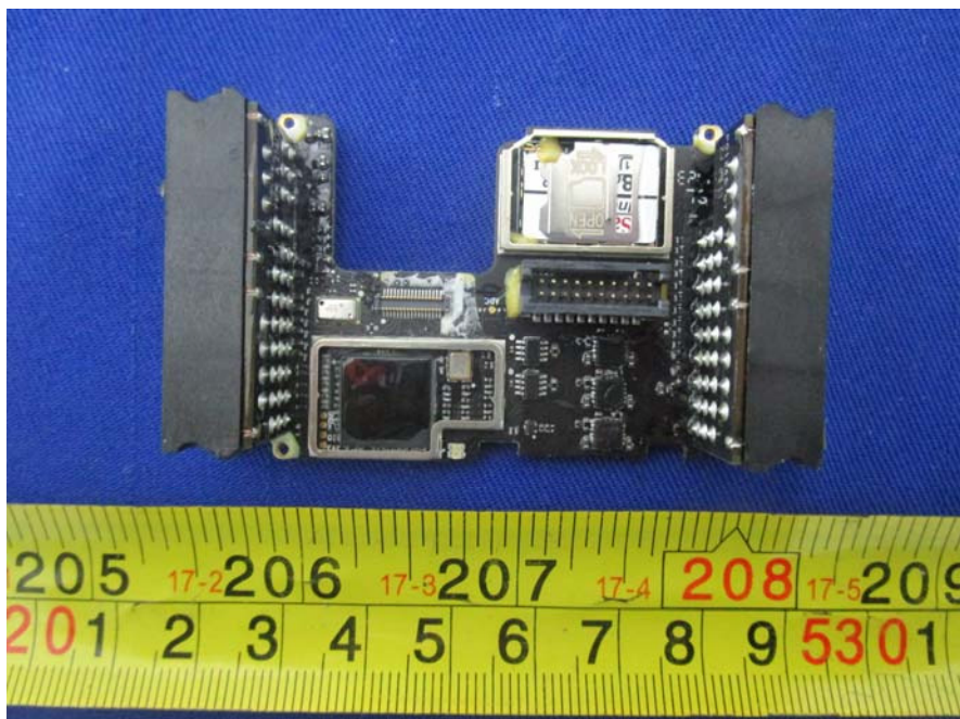
EUT – PCB-6 Top Uncover View
