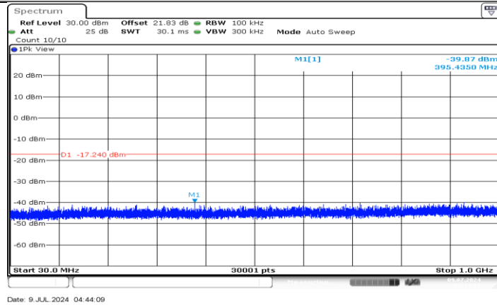
BLE_2M_Ant5_2440_30~1000
