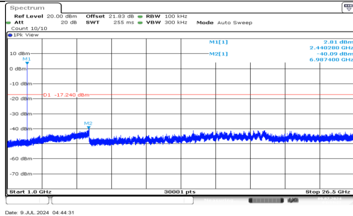
BLE_2M_Ant5_2440_1000~26500
