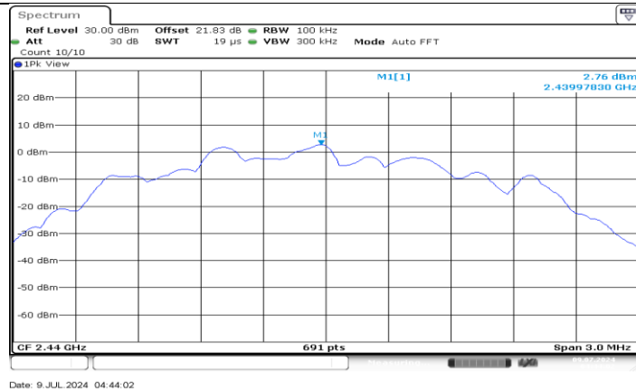
BLE_2M_Ant5_2440_0~Reference
