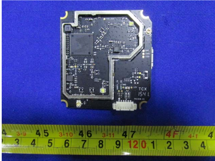
EUT –RF Module Top Uncover View
