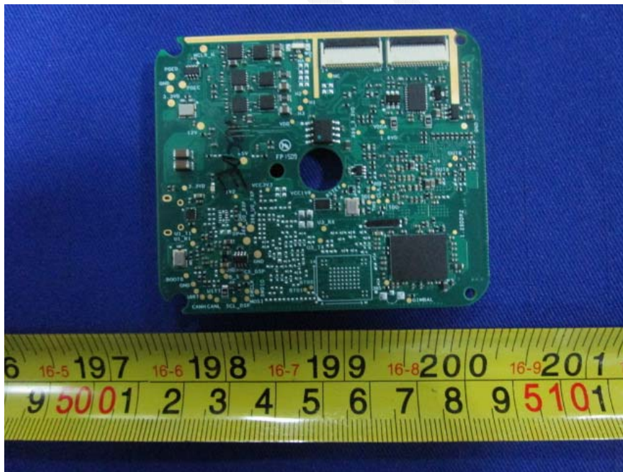
EUT –Main Camera Main Board Bottom View
