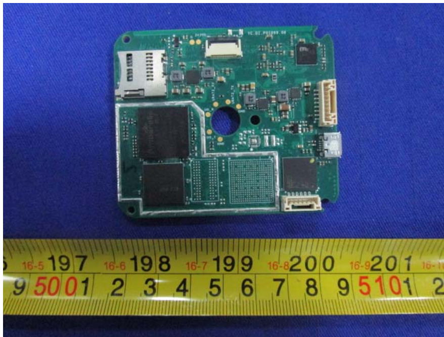
EUT –Main Camera Main Board Top View
