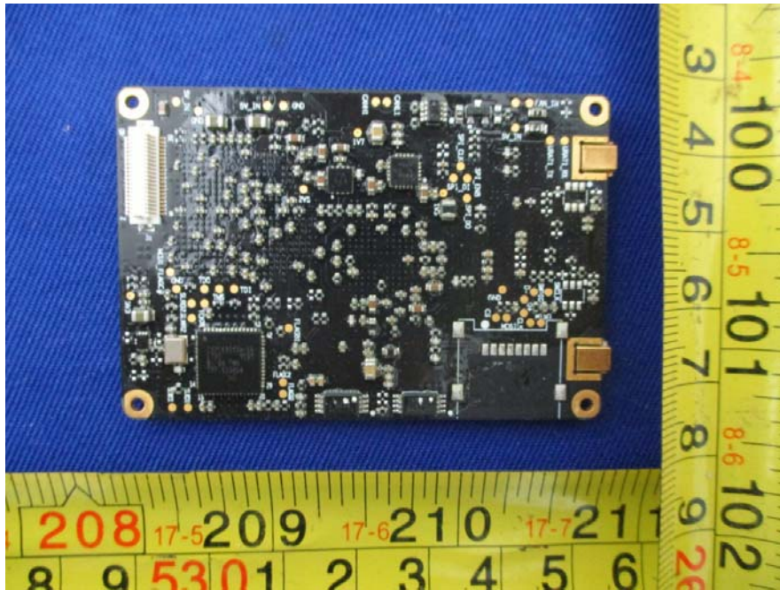
EUT – RF Module RF Board Bottom View
