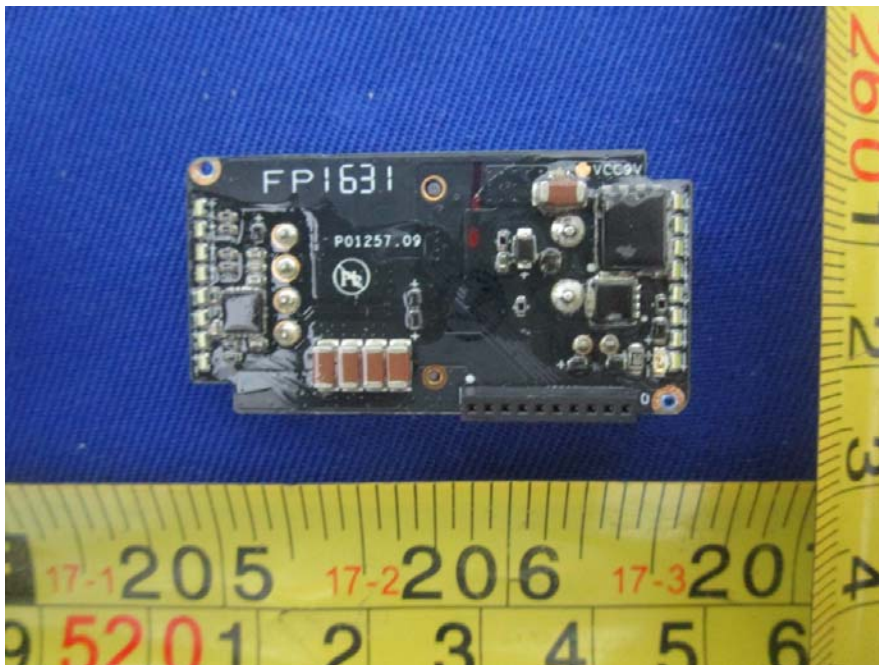
EUT – Flight Controller Module Sub-board-2 Bottom View
