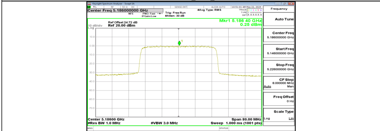
SRD 40MHz_Ant5_5186
