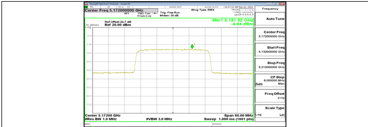
SRD 40MHz_Ant5_5172
