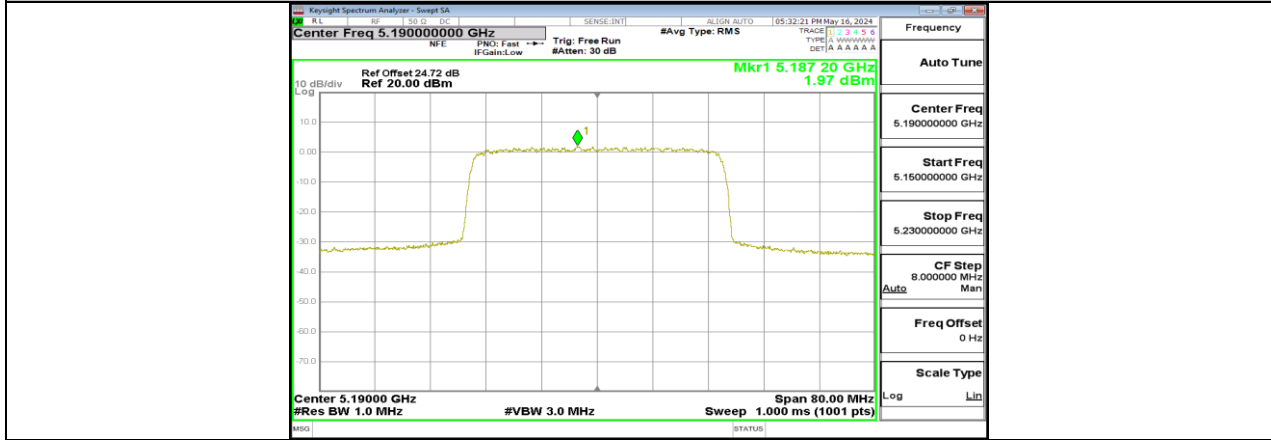
SRD 40MHz_Ant5_5190
