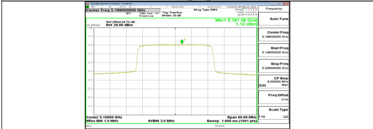
SRD 40MHz_Ant5_5188
