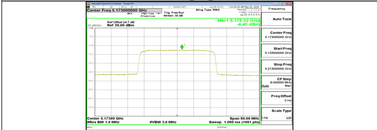
SRD 40MHz_Ant5_5173
