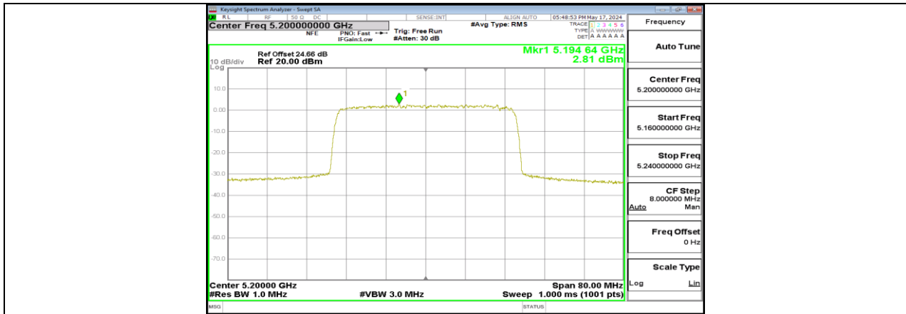
SRD 40MHz_Ant4_5200
