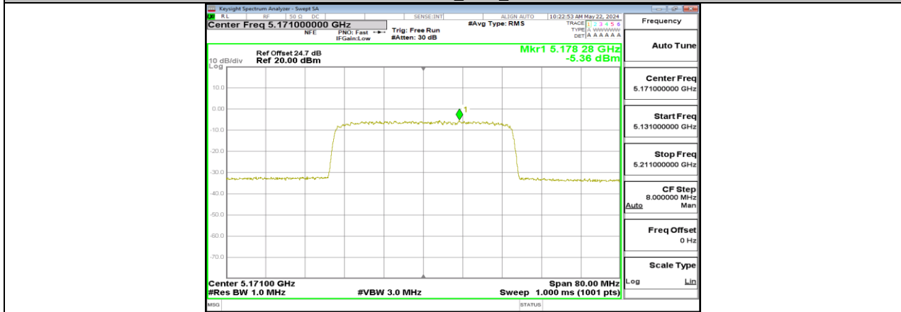
SRD 40MHz_Ant5_5171
