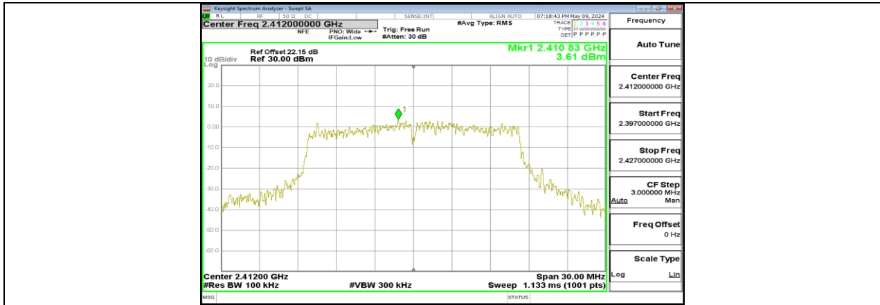
11G_Ant3_2412_0~Reference
