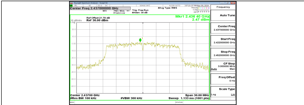
11G_Ant3_2437_0~Reference
