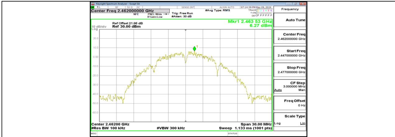
11B_Ant3_2462_0~Reference
