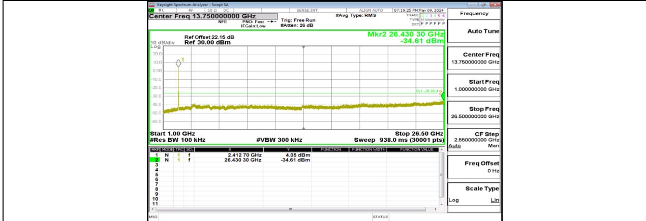
11G_Ant3_2412_1000~26500
