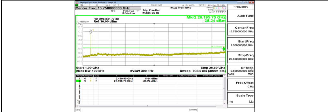
11G_Ant3_2437_1000~26500
