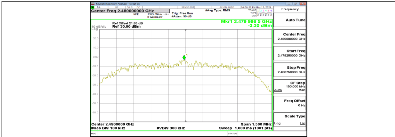
3DH5_Ant2_2480_0~Reference
