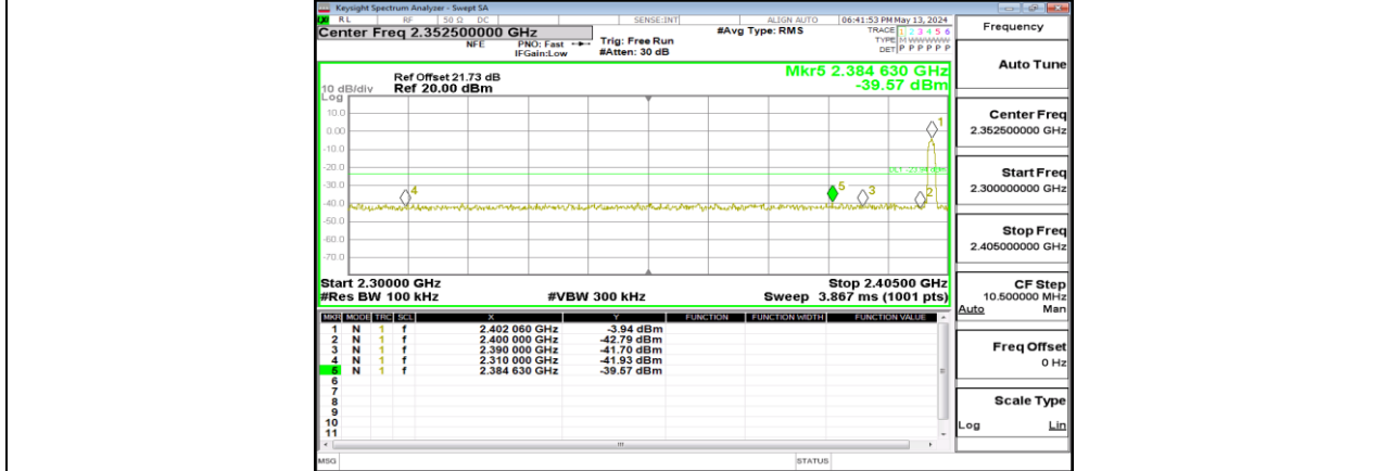
3DH5_Ant2_Low_2402
