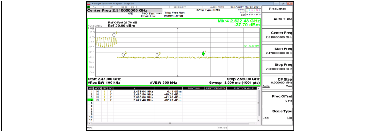
DH5_Ant2_High_Hop_2480
