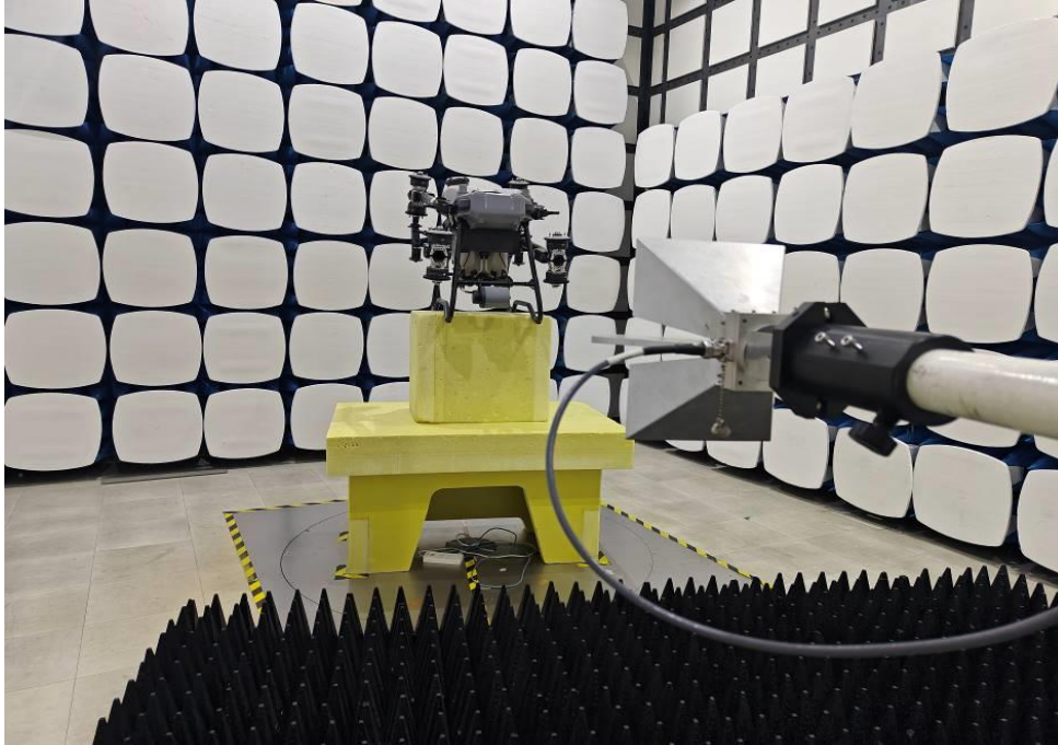
Radiated Emissions which fall in the restricted bands
