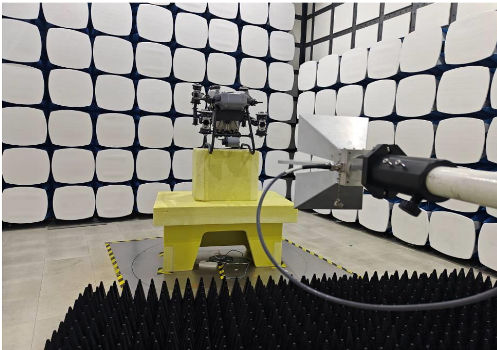
Radiated Spurious Emissions Above 1GHz
