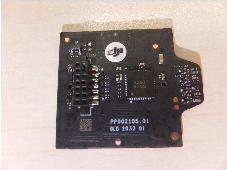
(TOF module 'Dot-Matrix Display & Distance Sensing')
