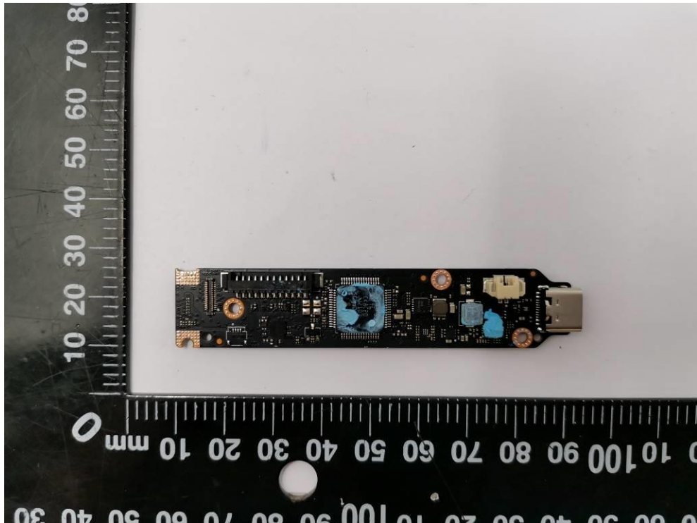
Fig.8. PCB view 1
