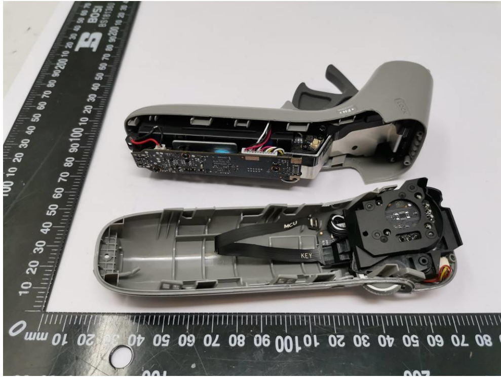
Fig.1. Internal view 1
