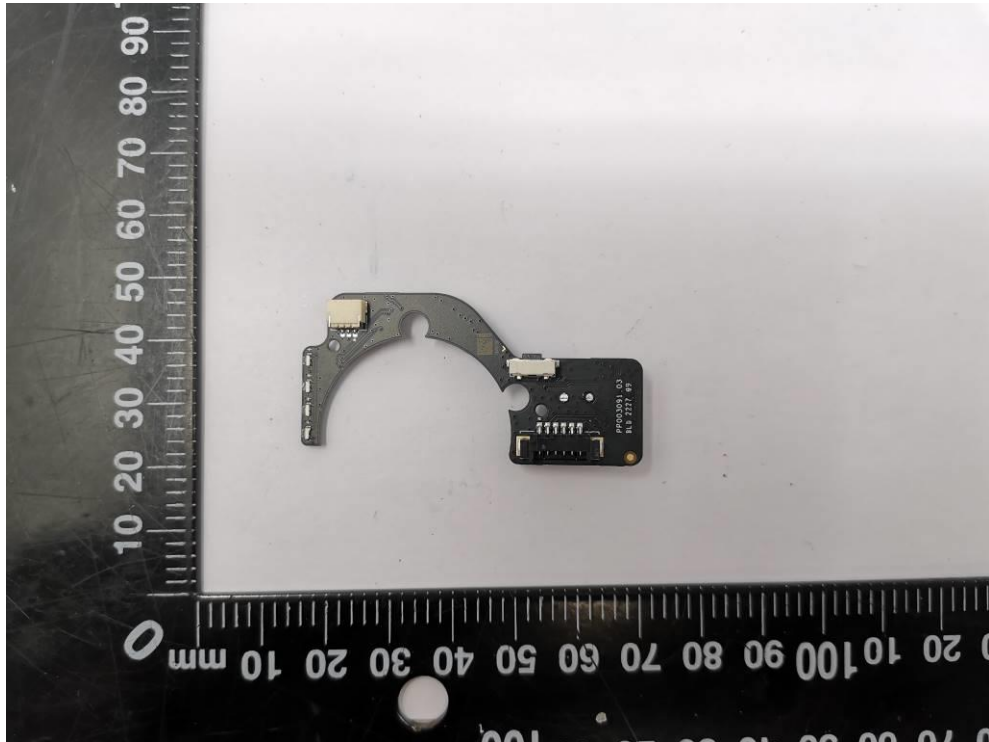
Fig.13. PCB view 6
