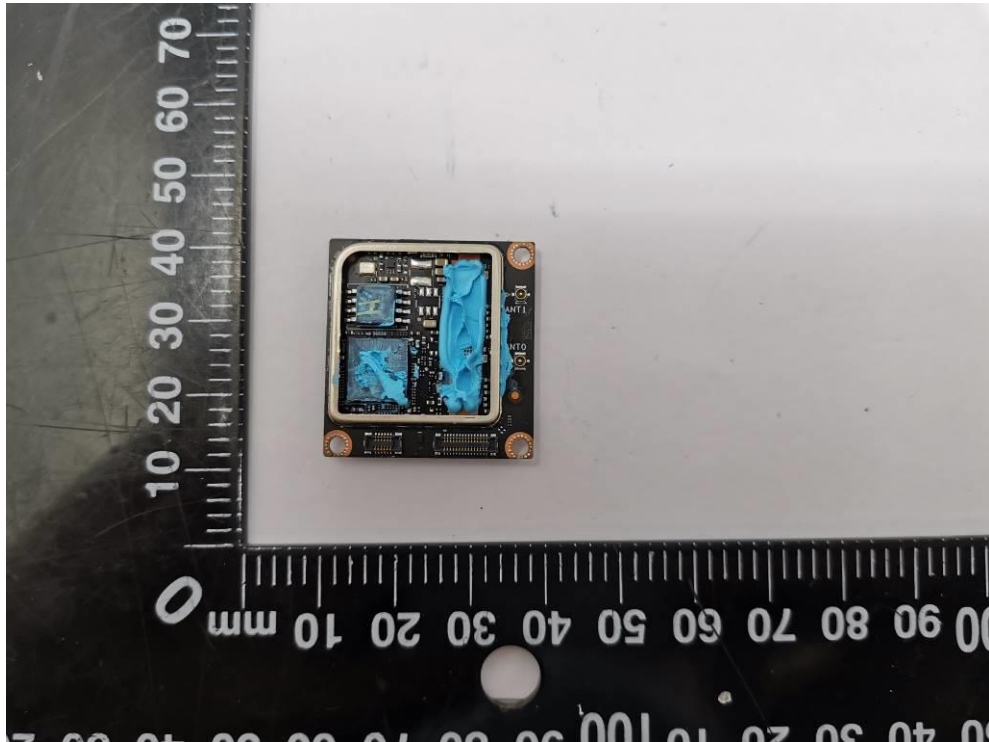
Fig.11. PCB view 4
