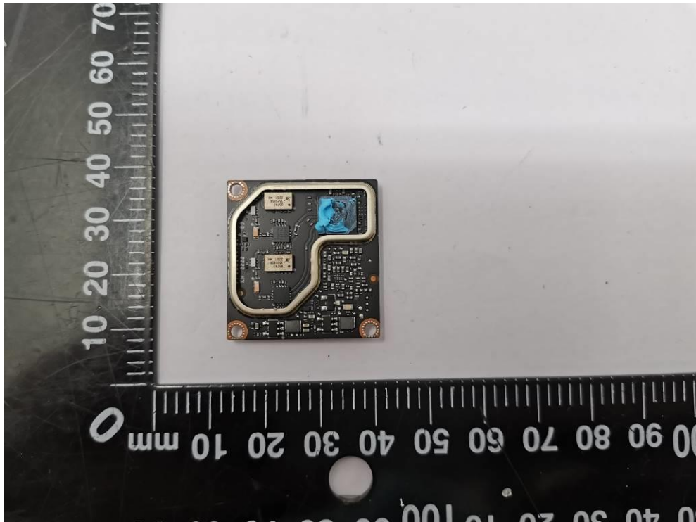
Fig.10. PCB view 3
