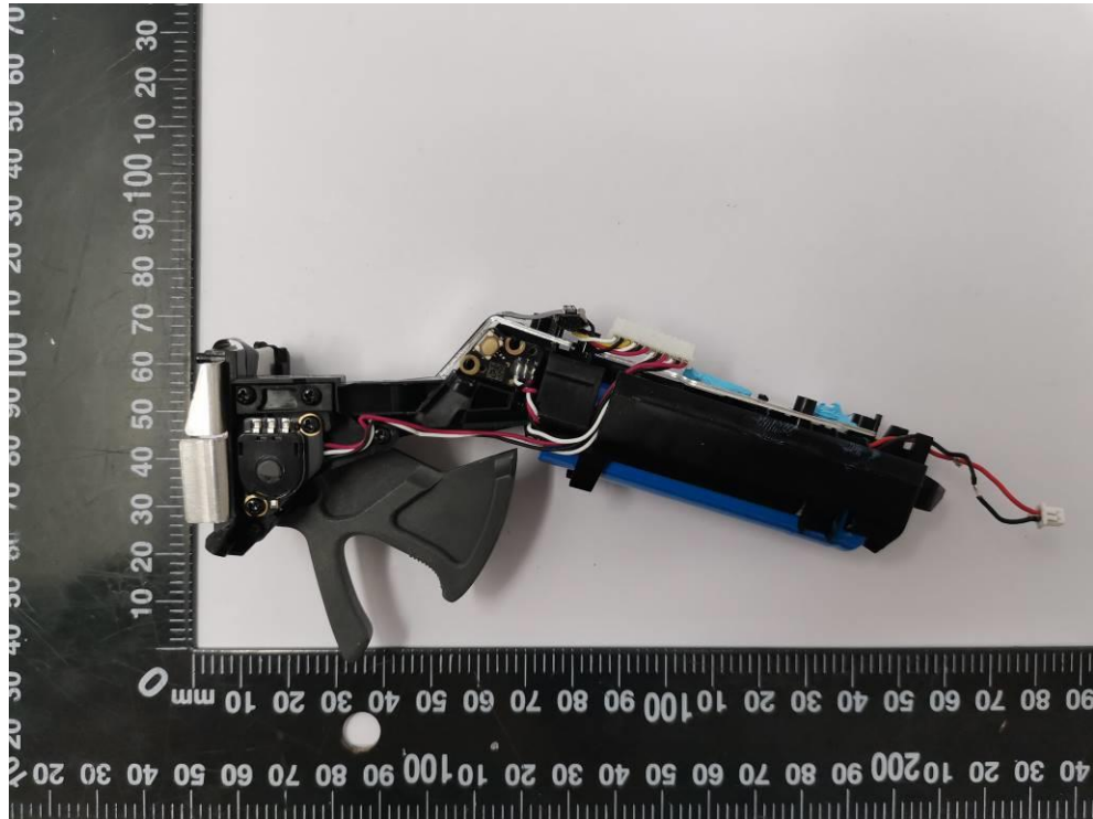
Fig.5. Internal view 5
