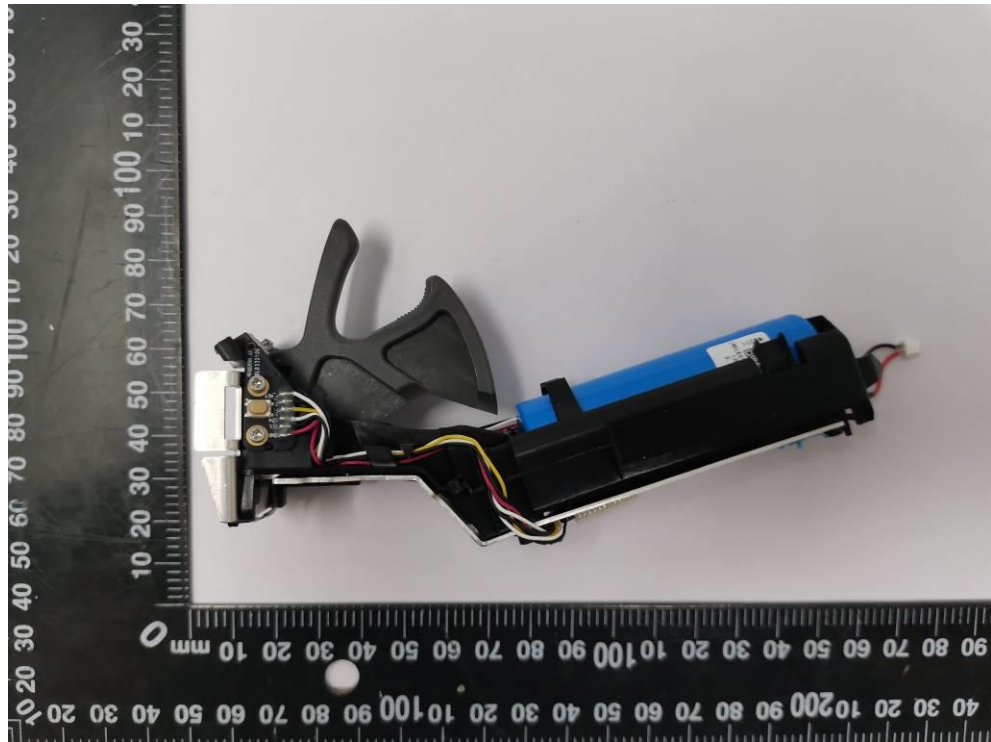
Fig.6. Internal view 6
