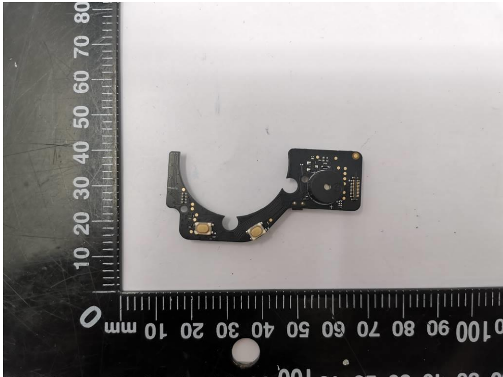
Fig.12. PCB view 5
