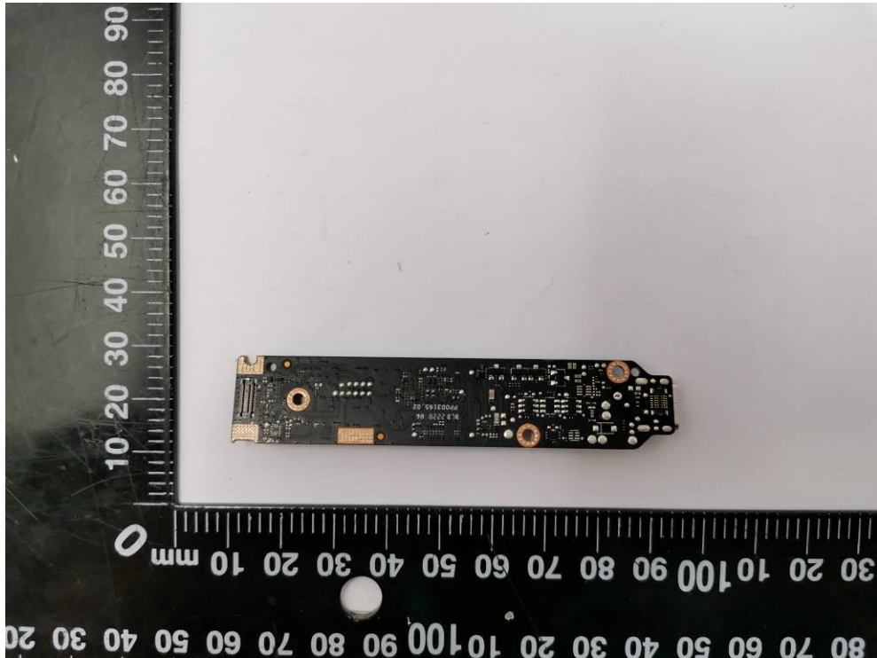
Fig.9. PCB view 2
