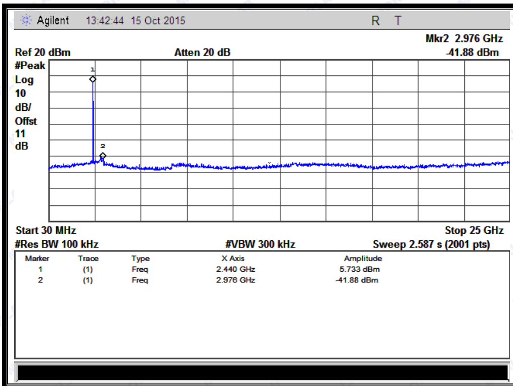
(Plot B.1: Channel = 15, 30MHz to 25GHz)
