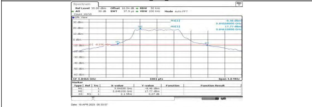
1.4 MHz Ant1 5846.5
