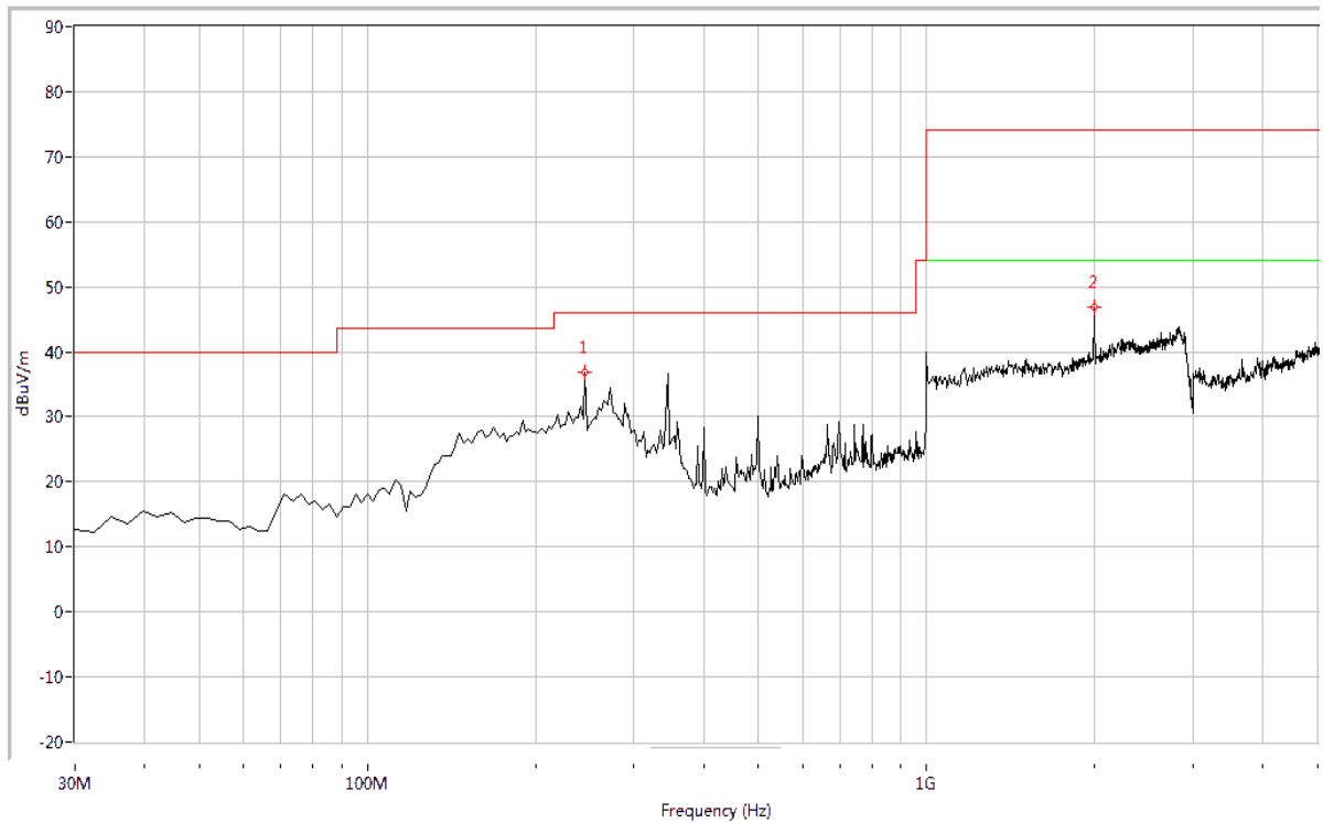
(Plot C: 30MHz – 5GHz, Test Antenna Horizontal)
