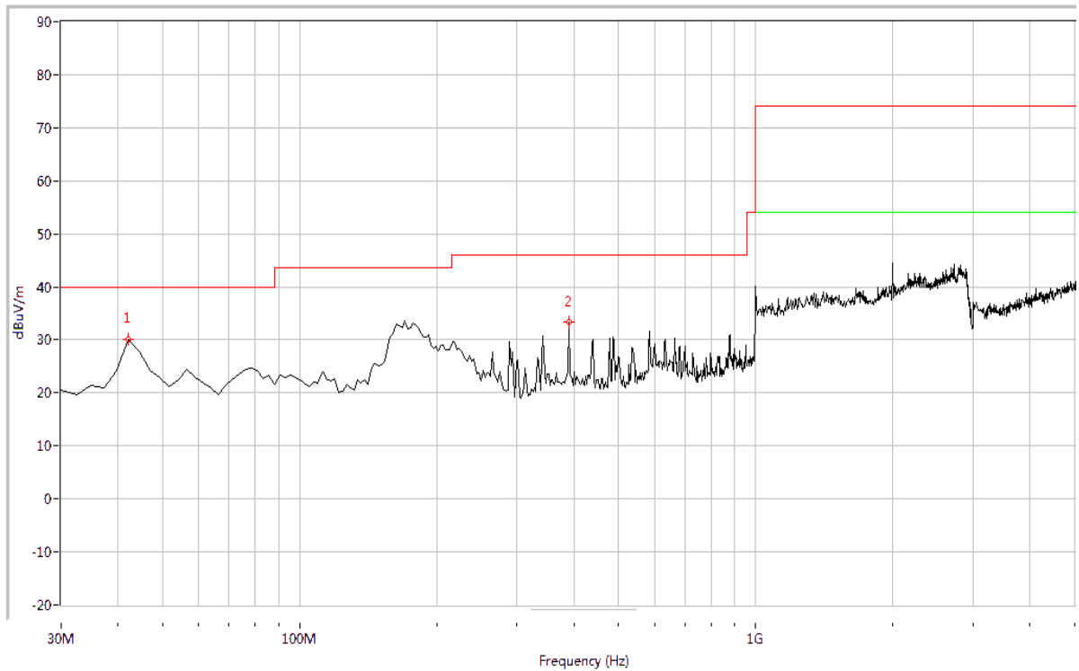
(Plot B: 30MHz – 5GHz, Test Antenna Vertical)
