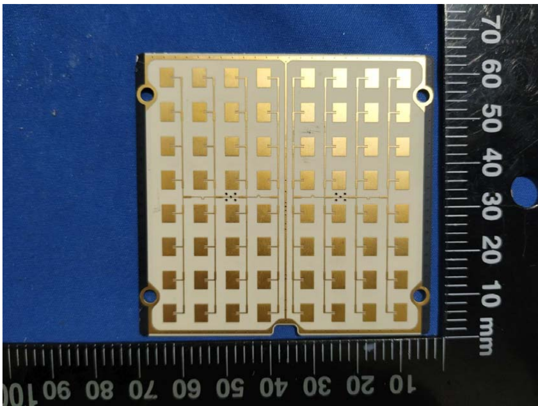
Directional antenna
