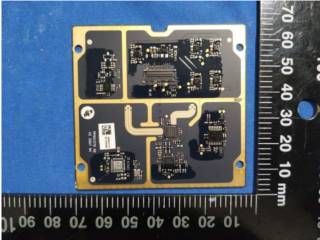
Directional antenna
