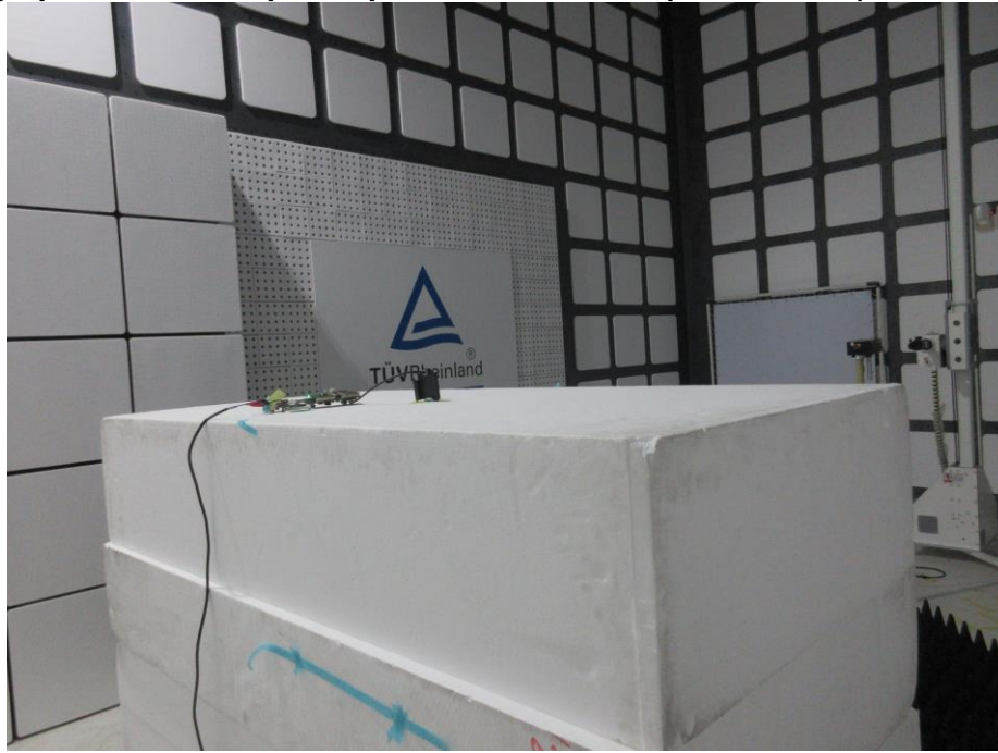
Photograph 9: Test Setup for Spurious Emissions (Back View 7)
