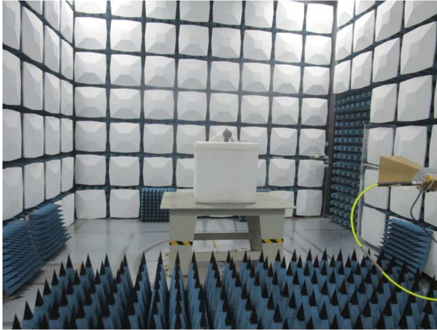
Radiated Emission 18 GHz-40GHz View
