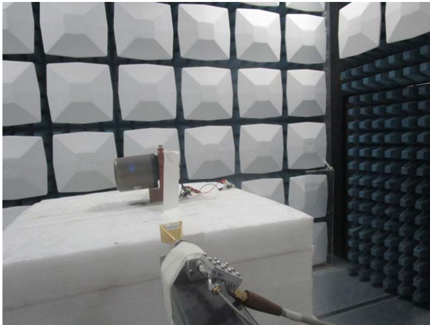
Radiated Emission 40GHz-100GHz View
