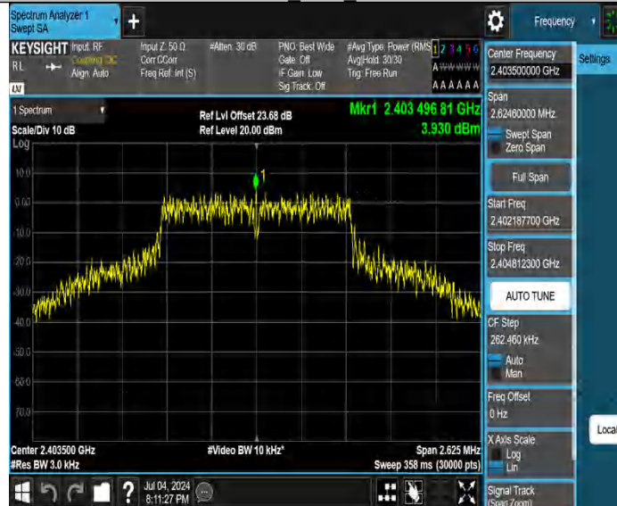
1.4MHz Ant6 2403.5
