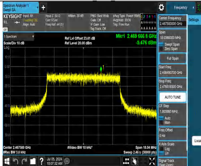
10MHz Ant6 2467.5
