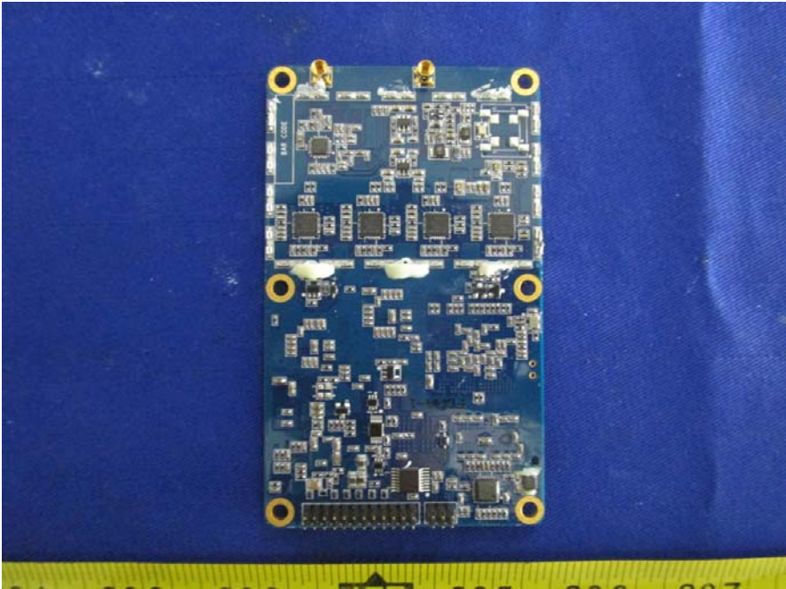
EUT- RTK Board Bottom View
