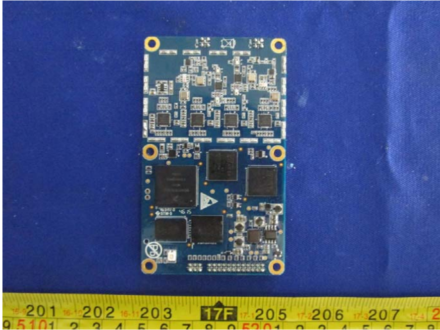
EUT- RTK Board Top View
