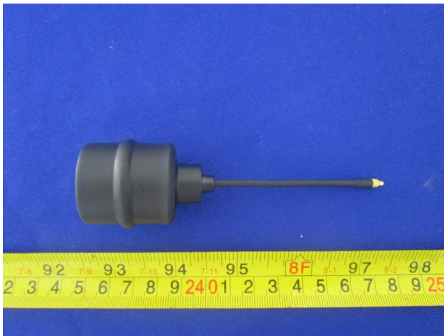
EUT –Cylindrical Antenna View
