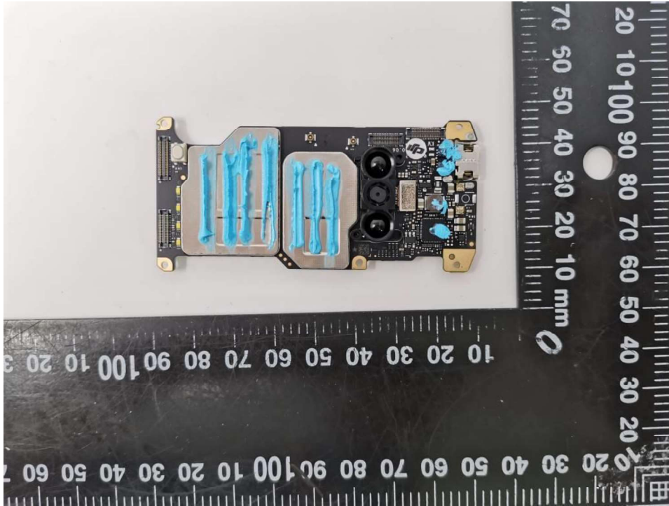
Figure 9: Mainboard view -1
