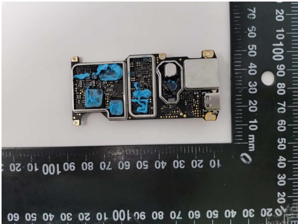
Figure 12: Mainboard view -4
