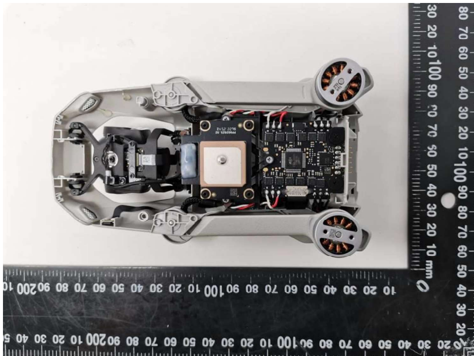
Figure 6: Internal view – 1 (with top cover removed)
