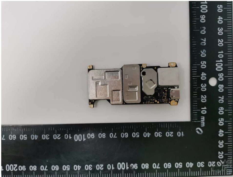
Figure 11: Mainboard view -3
