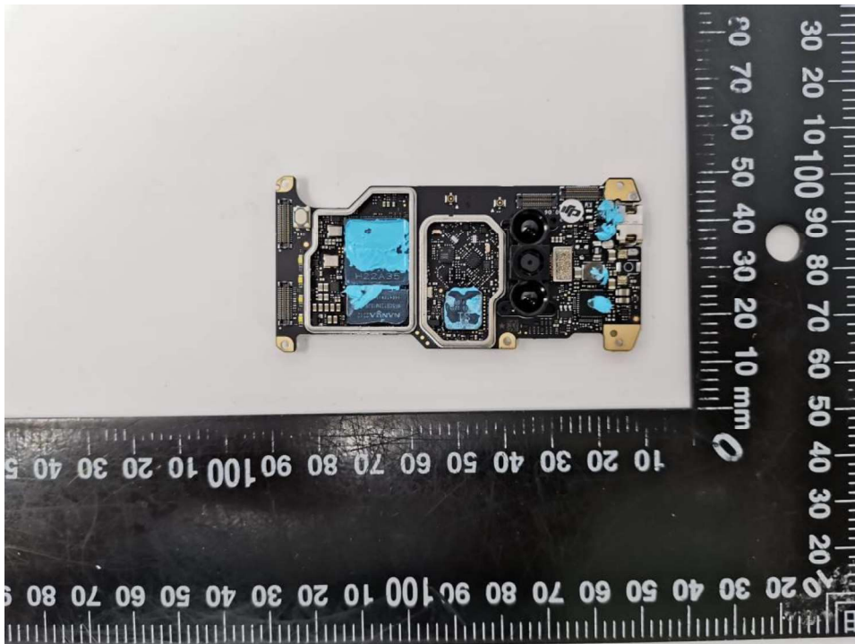
Figure 10: Mainboard view -2
