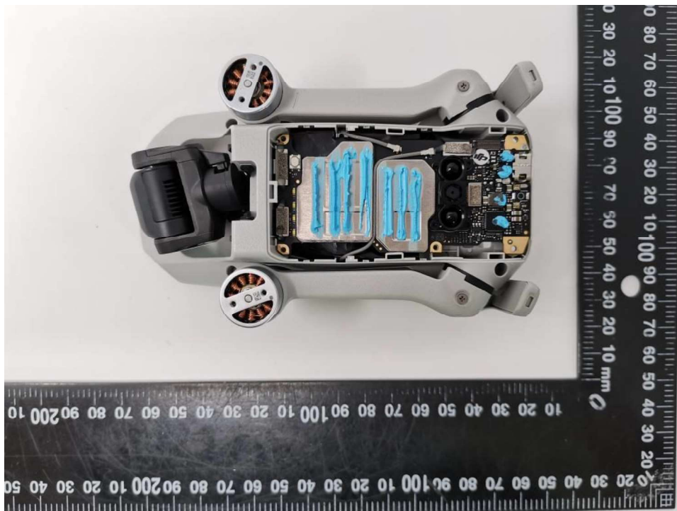
Figure 8: Internal view - 3
