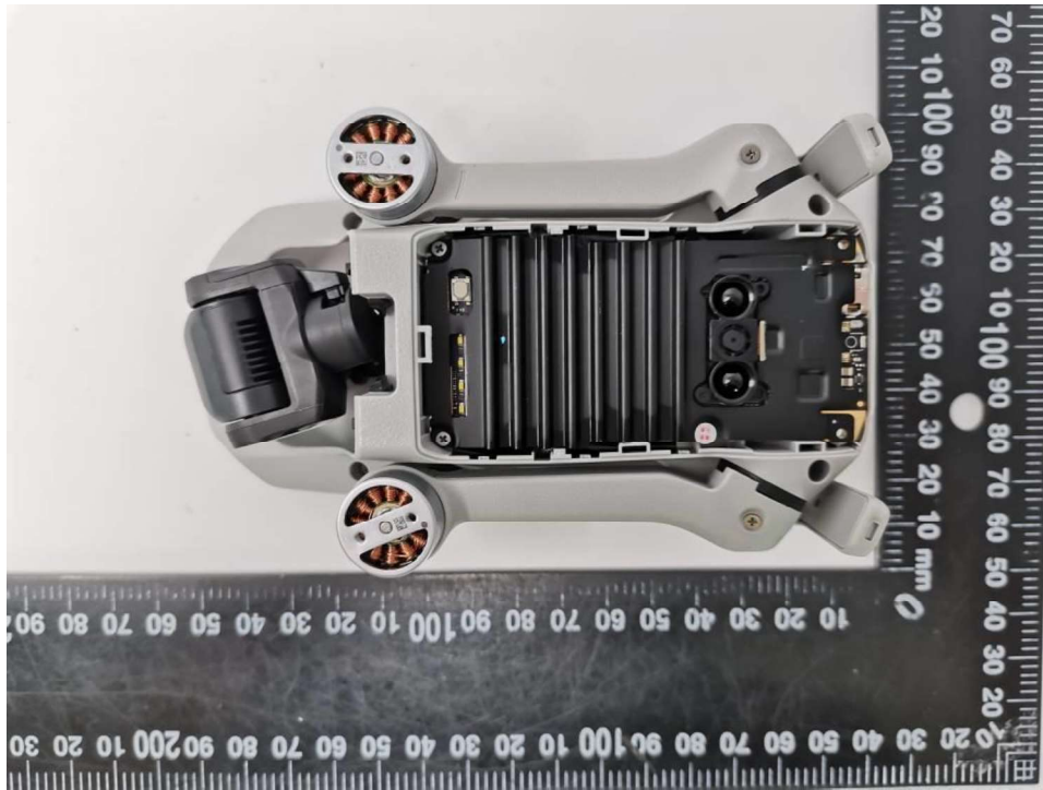
Figure 7: Internal view – 2 (with bottom cover removed)
