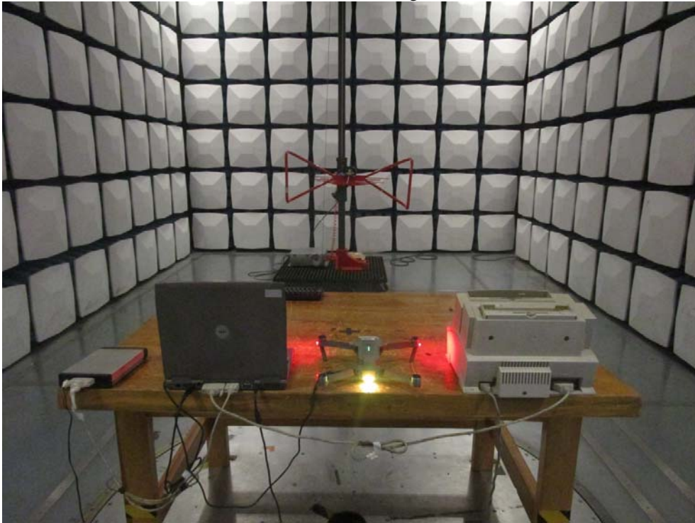
RE Below 1G-downloading-rear View
