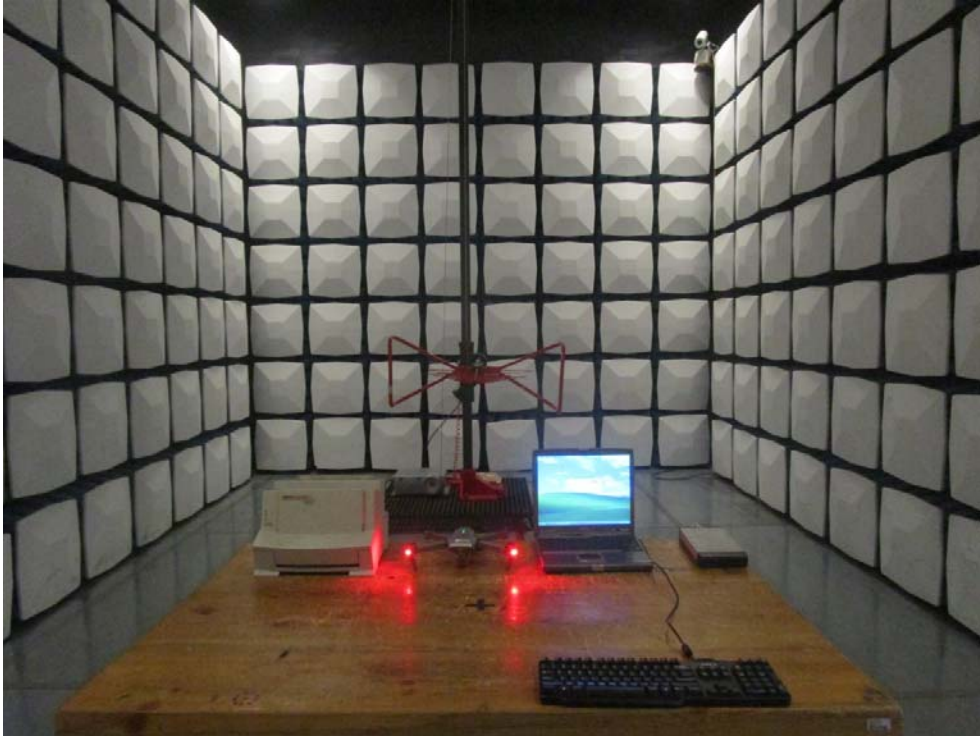
RE Below 1G-downloading-front View
