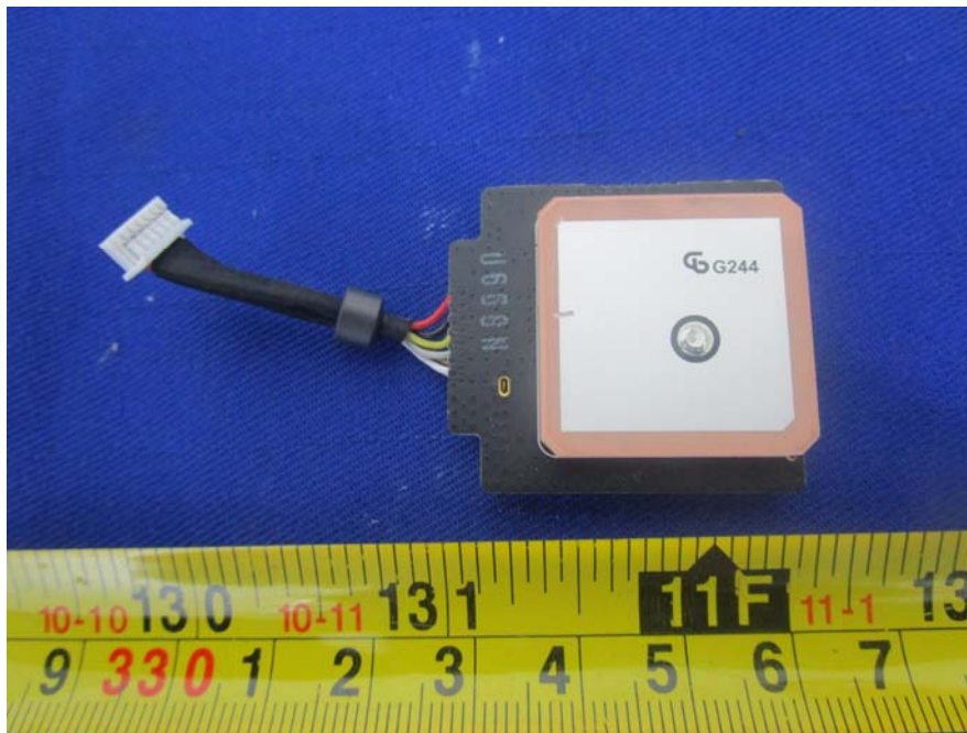
EUT –GPS Module Bottom&Antenna View
