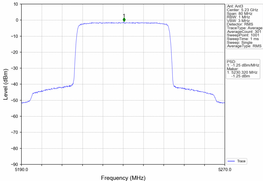
40_HCH_5230MHz_Ant3_NTNV
