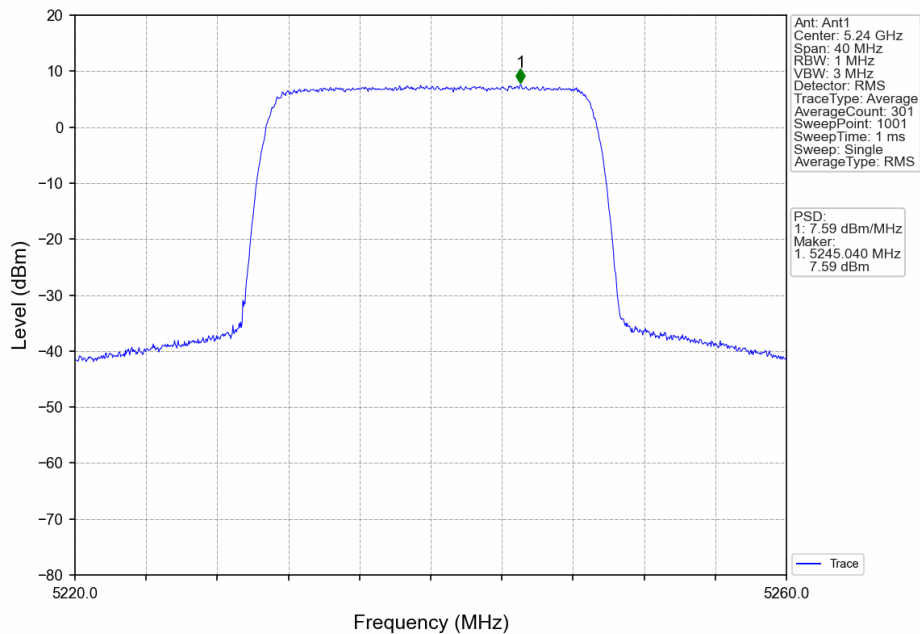
20_HCH_5240MHz_Ant1_NTNV
