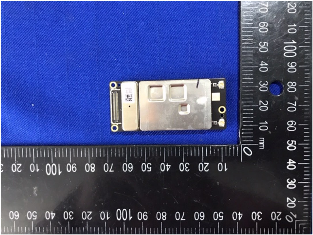
RF Board
