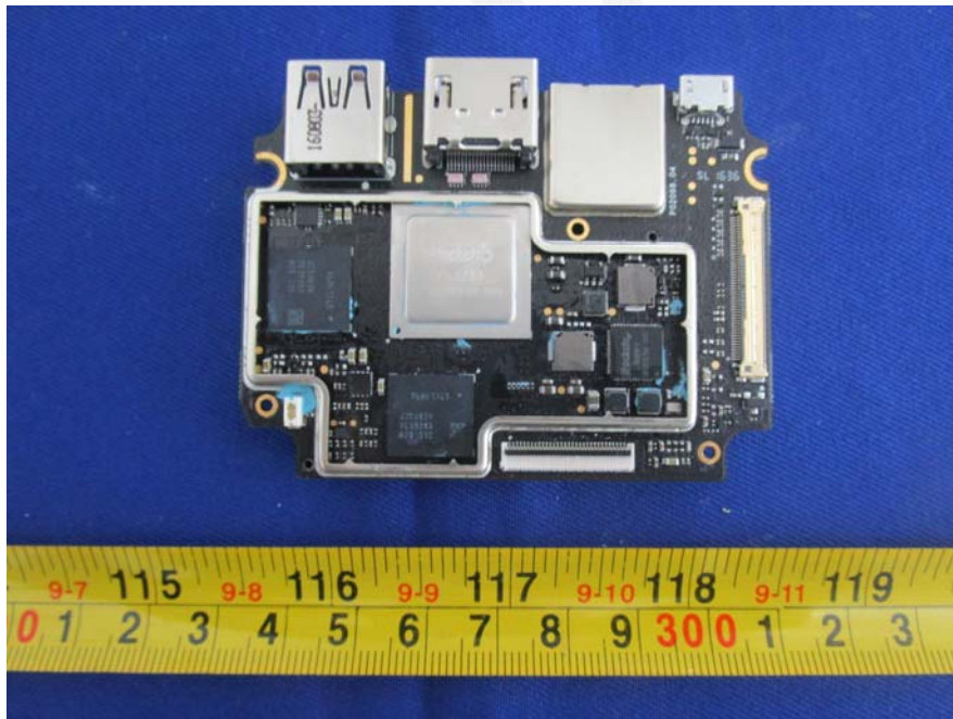
EUT – Unshielded Board #1 Top View
