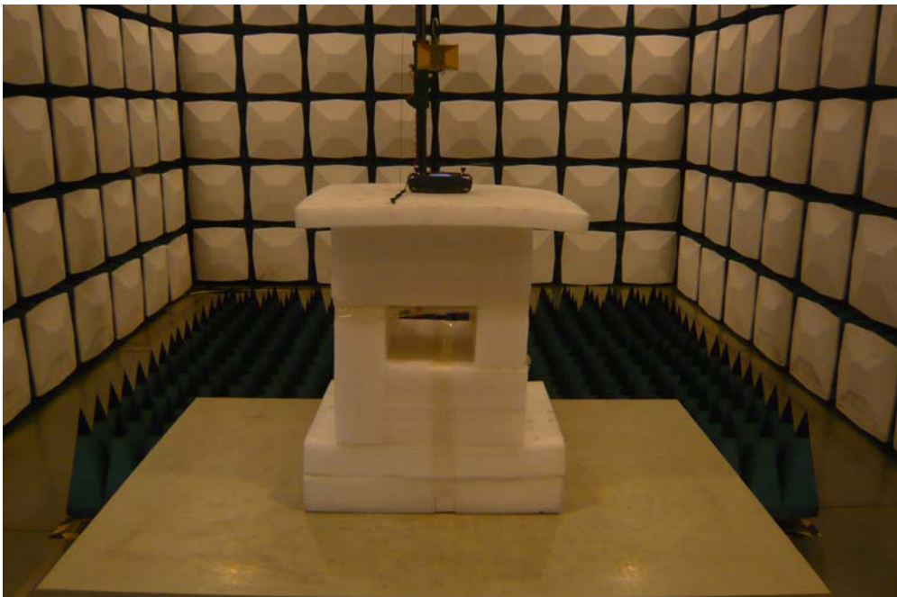
Radiated Emission Above 1GHz View
