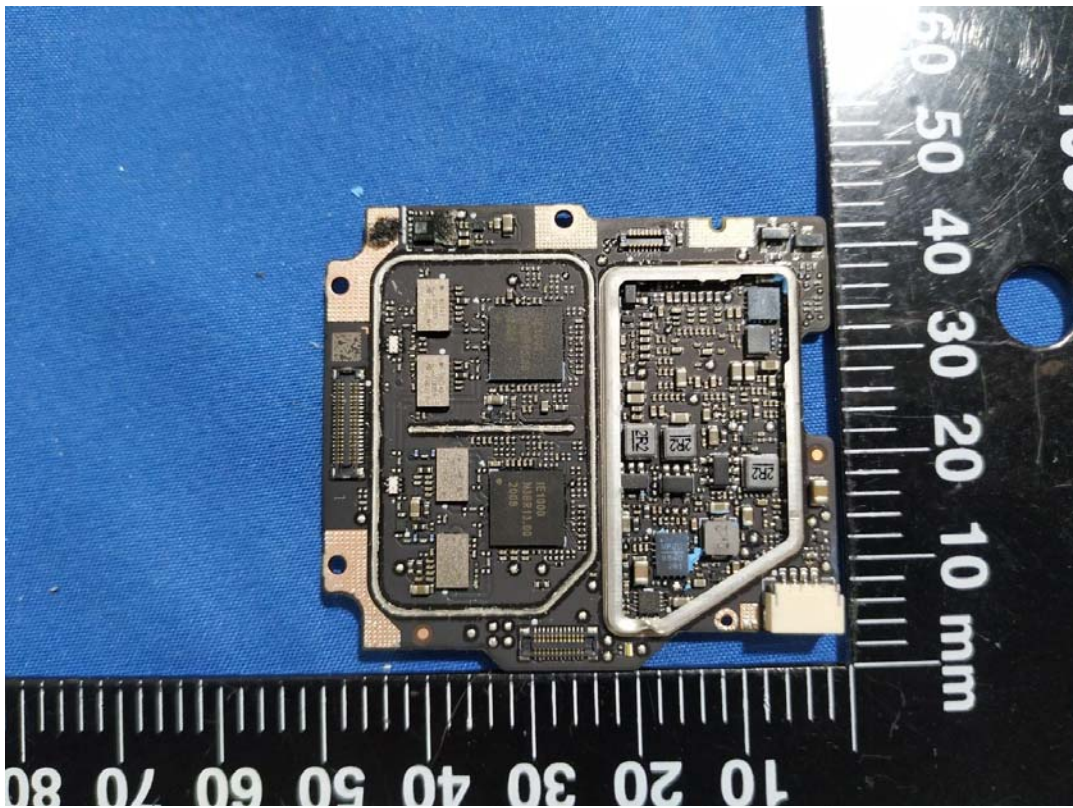
ADS-B Board
