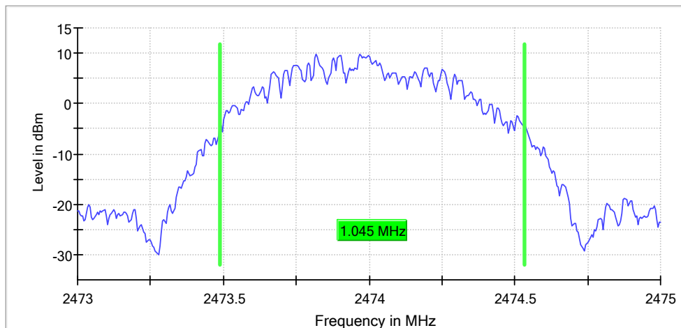
99 % Bandwidth
