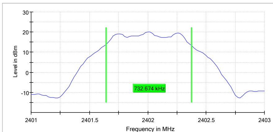
6 dB Bandwidth
