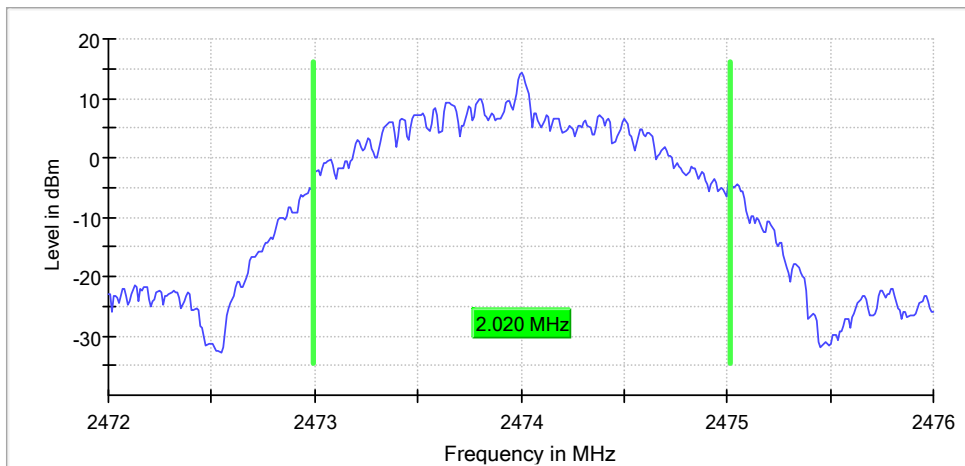
99 % Bandwidth
