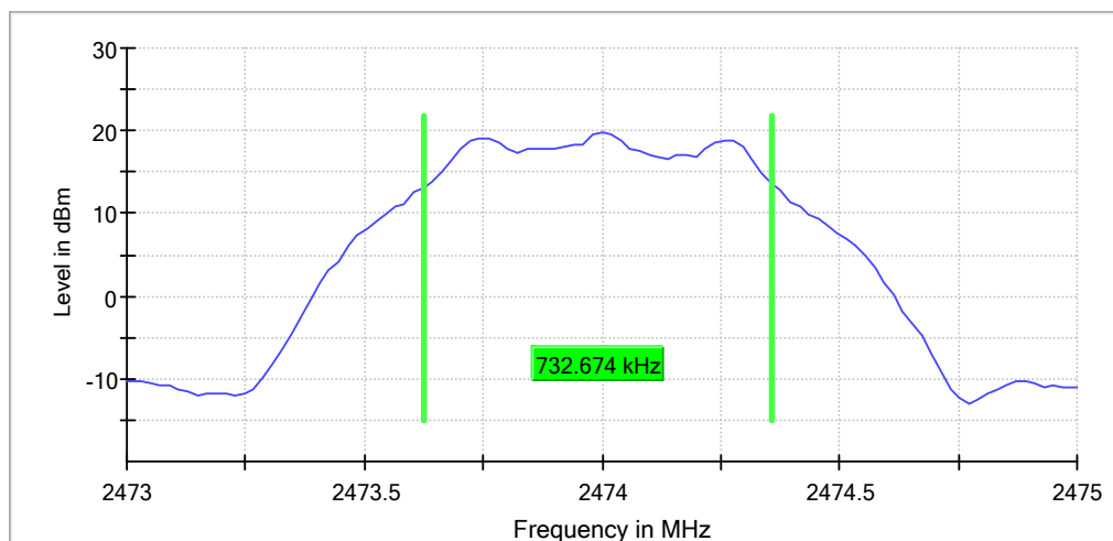
6 dB Bandwidth
