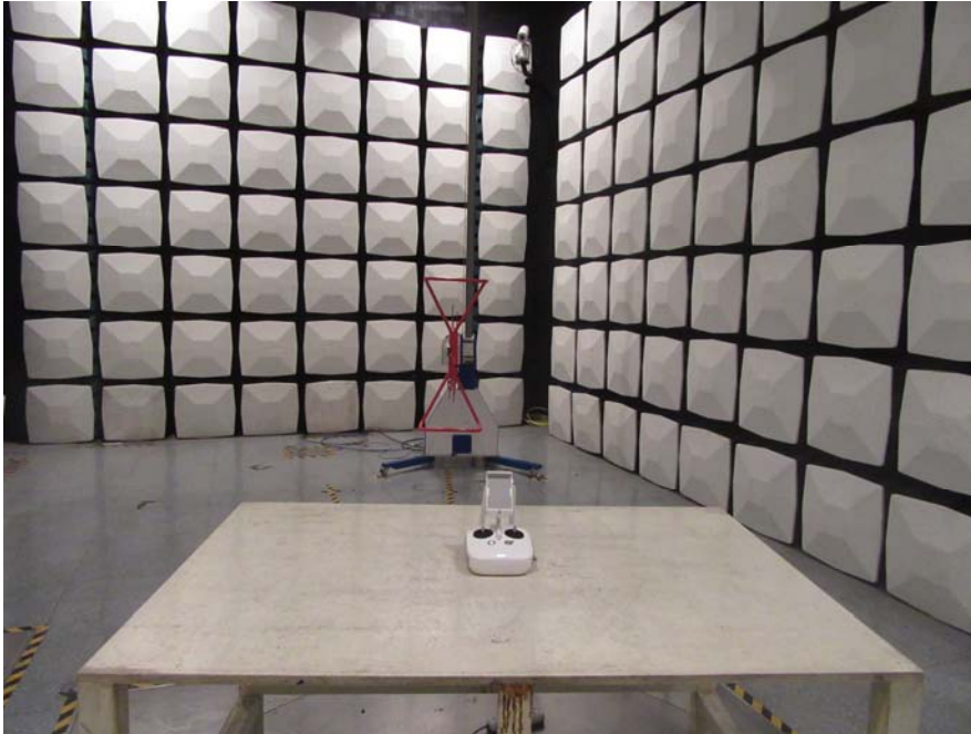
Radiated Emission Below 1GHz View - Operating
