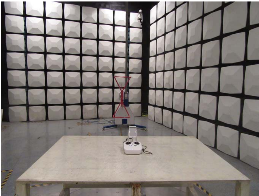
Radiated Emission Below 1GHz View - Charging
