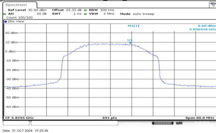
SDR 40M_Ant1_5829.5
