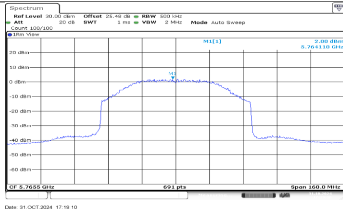
SDR 80M_Ant2_5765.5
