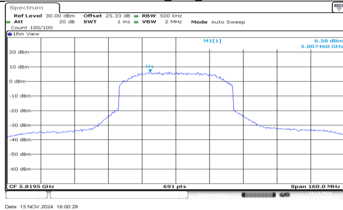
SDR 60M_Ant1_5819.5
