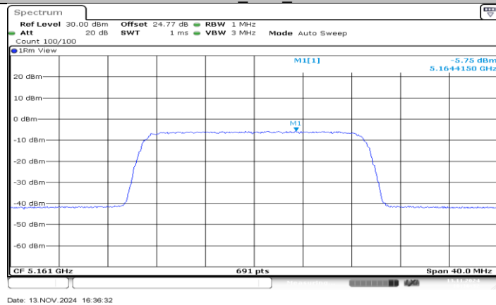
SDR 20M_Ant1_5161
