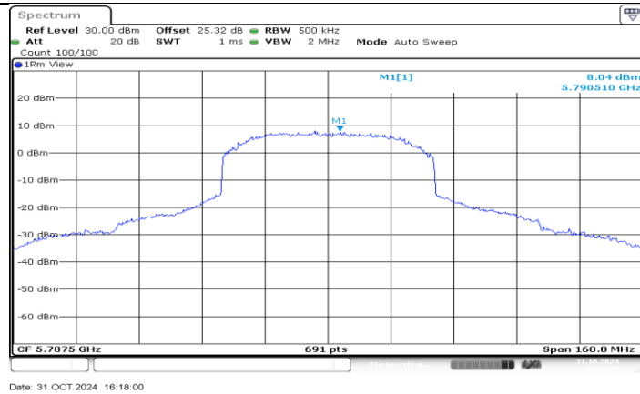
SDR 60M_Ant1_5787.5
