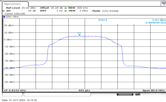
SDR 40M_Ant2_5812.5
