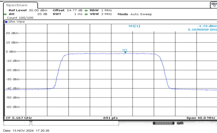
SDR 20M_Ant1_5167
