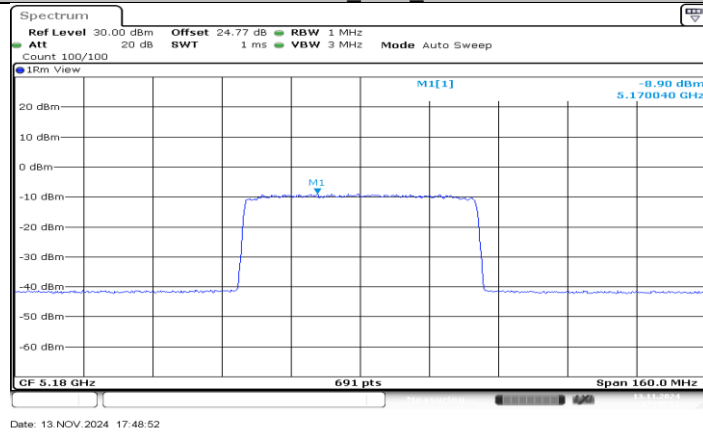
SDR 60M_Ant2_5180
