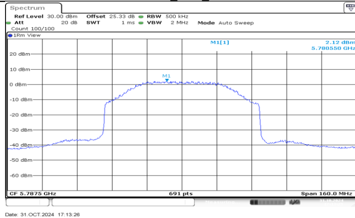
SDR 80M_Ant2_5787.5
