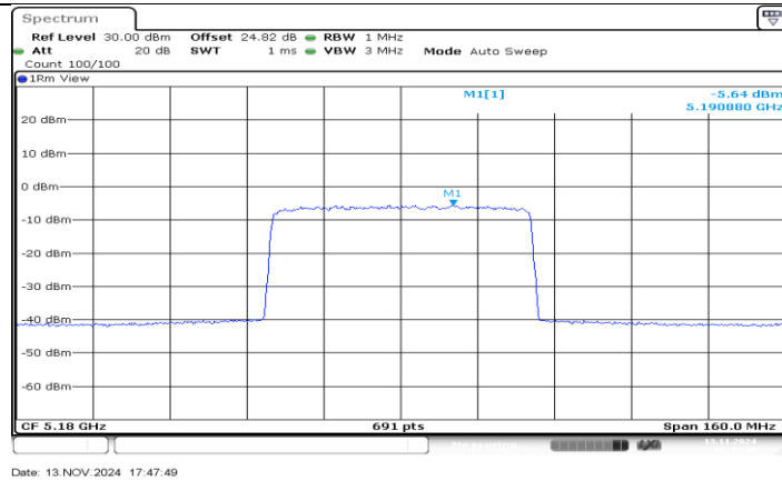
SDR 60M_Ant1_5180
