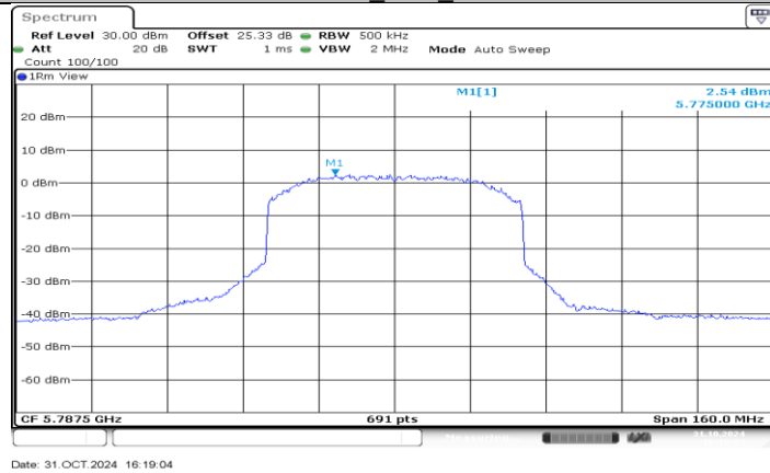
SDR 60M_Ant2_5787.5
