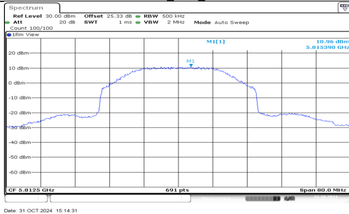
SDR 40M_Ant1_5812.5
