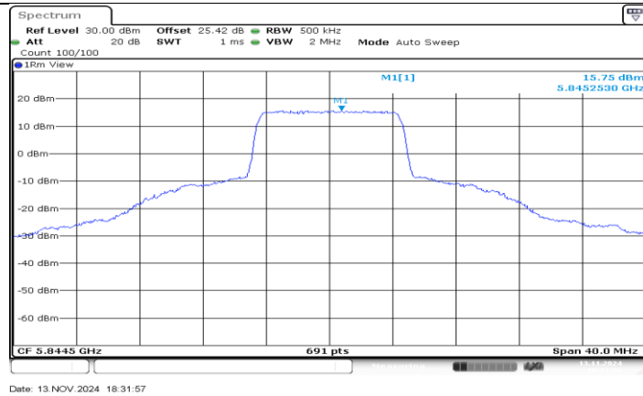
SDR 10M_Ant1_5844.5
