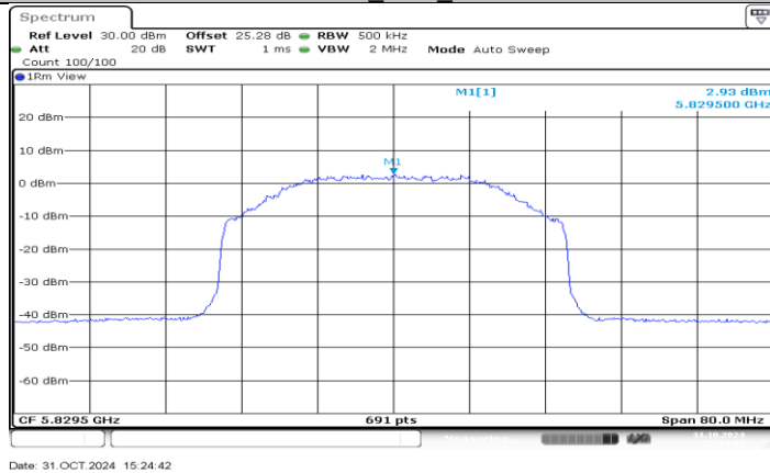
SDR 40M_Ant2_5829.5
