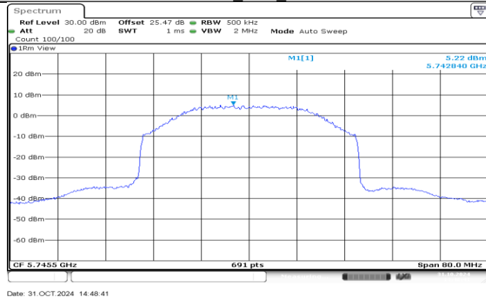
SDR 40M_Ant2_5745.5
