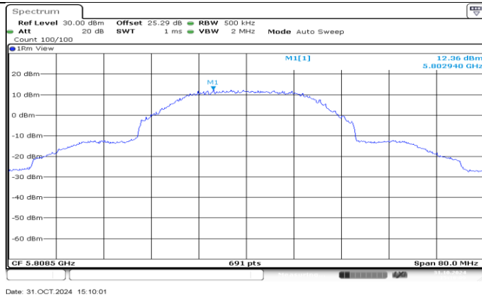
SDR 40M_Ant1_5808.5
