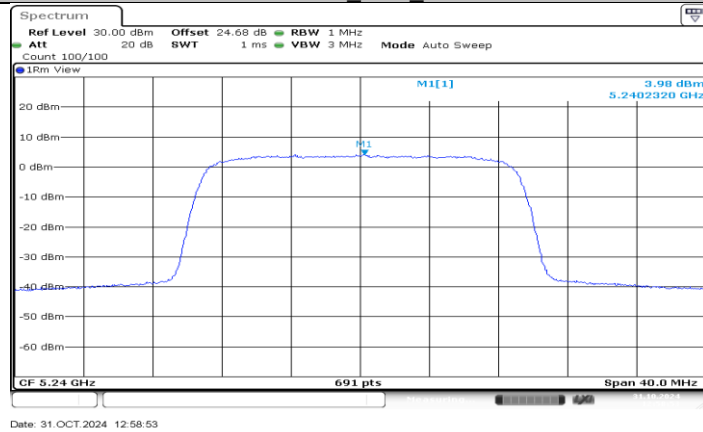
SDR 20M_Ant2_5240
