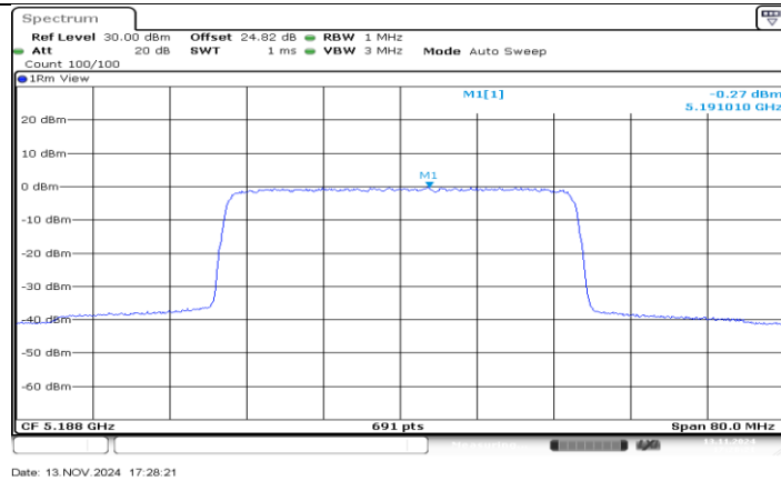
SDR 40M_Ant1_5188
