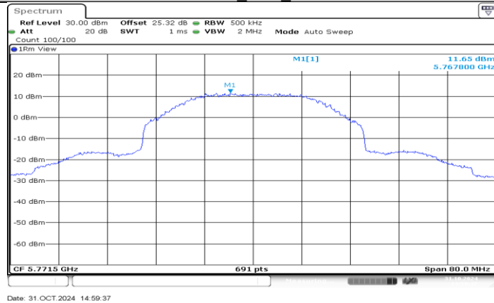
SDR 40M_Ant1_5771.5
