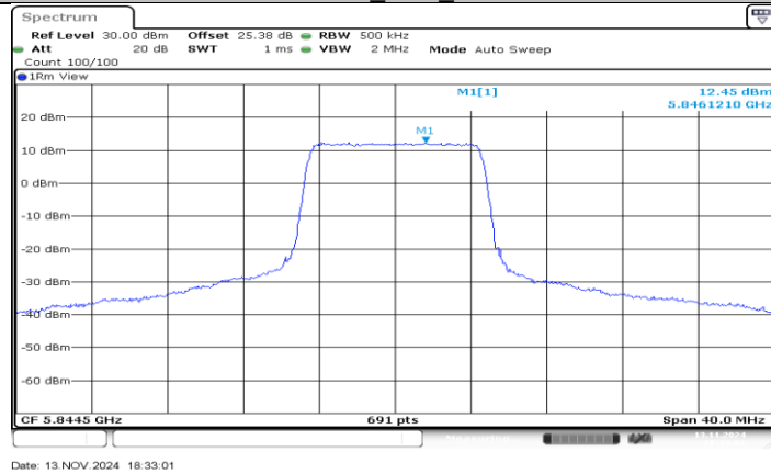
SDR 10M_Ant2_5844.5
