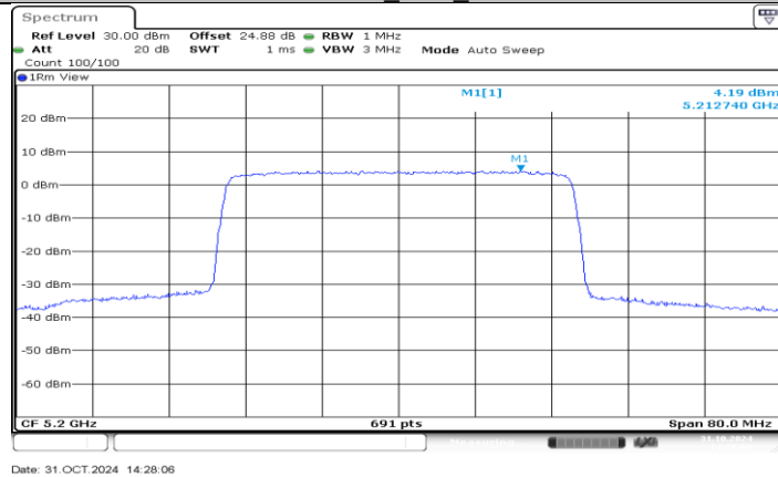
SDR 40M_Ant1_5200
