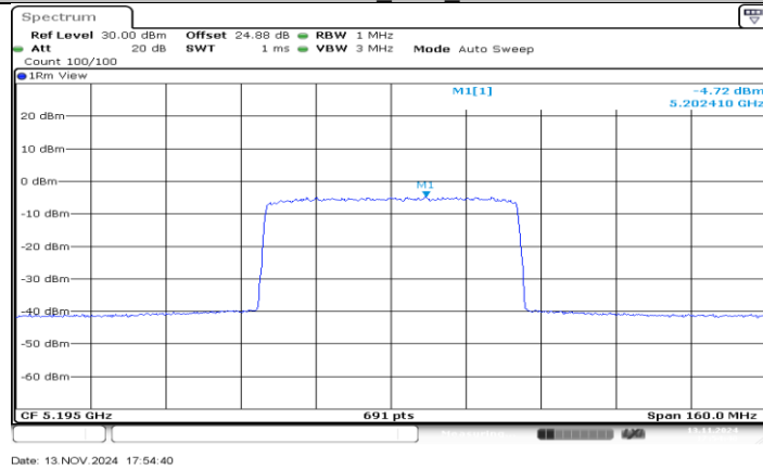
SDR 60M_Ant1_5195
