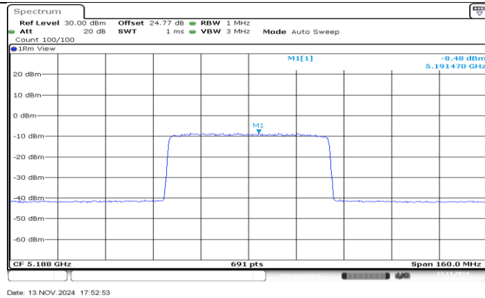
SDR 60M_Ant2_5188
