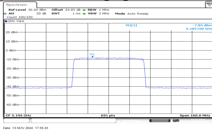
SDR 60M_Ant2_5195
