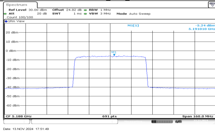
SDR 60M_Ant1_5188
