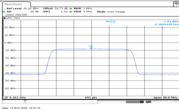
SDR 20M_Ant2_5161
