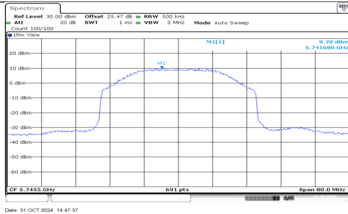
SDR 40M_Ant1_5745.5
