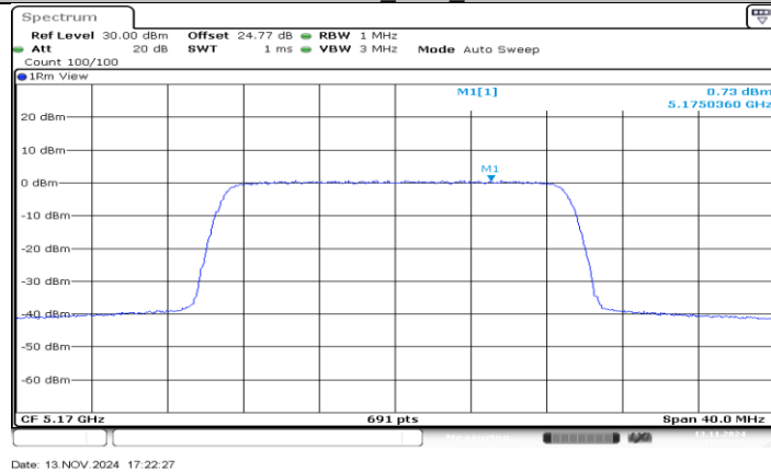
SDR 20M_Ant1_5170
