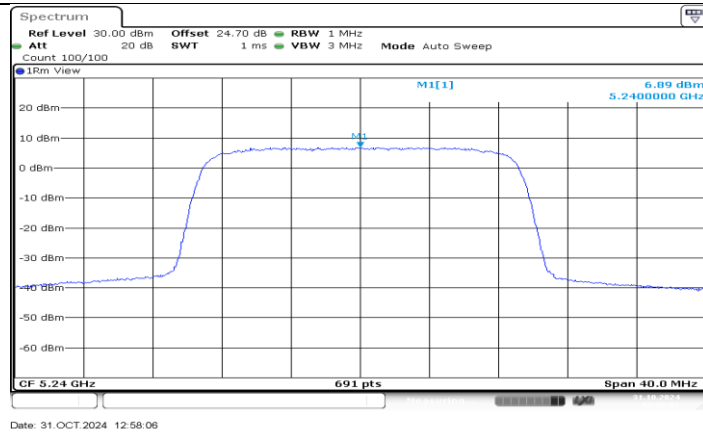
SDR 20M_Ant1_5240
