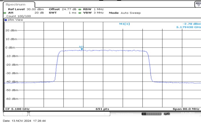
SDR 40M_Ant2_5188
