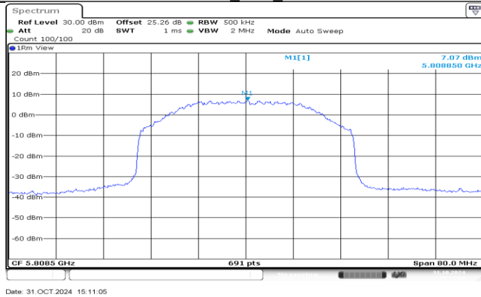
SDR 40M_Ant2_5808.5
