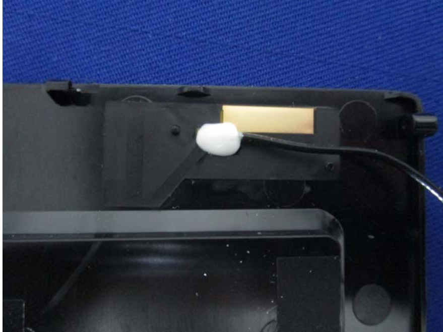
EUT –Wifi Antenna-Chain 1 View
