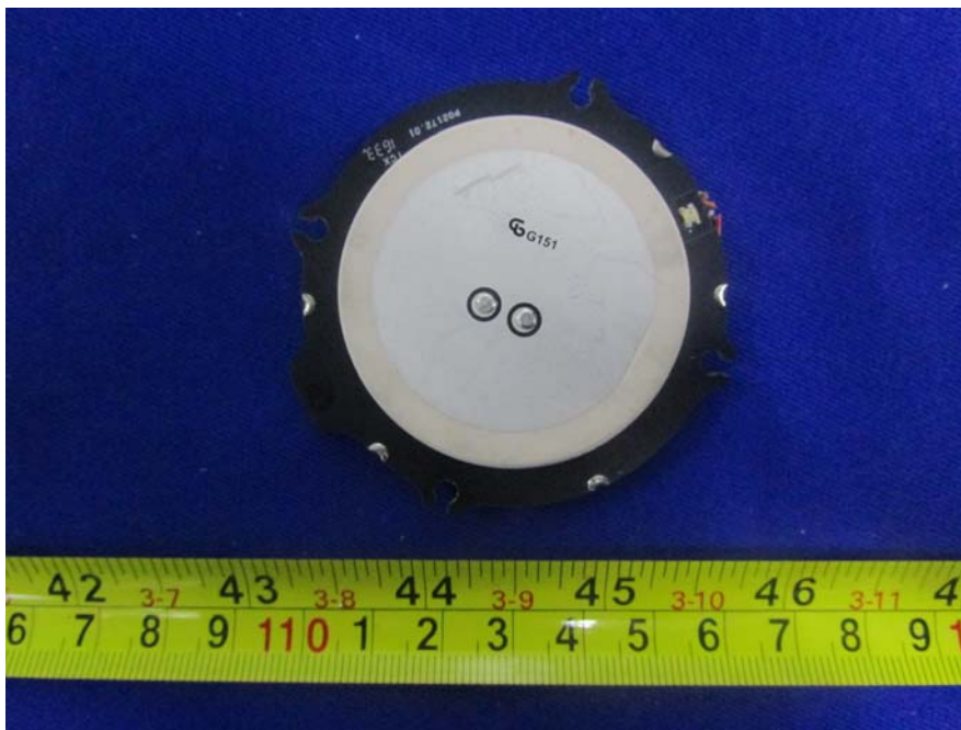
EUT-GPS Module-2 Bottom and Antenna View
