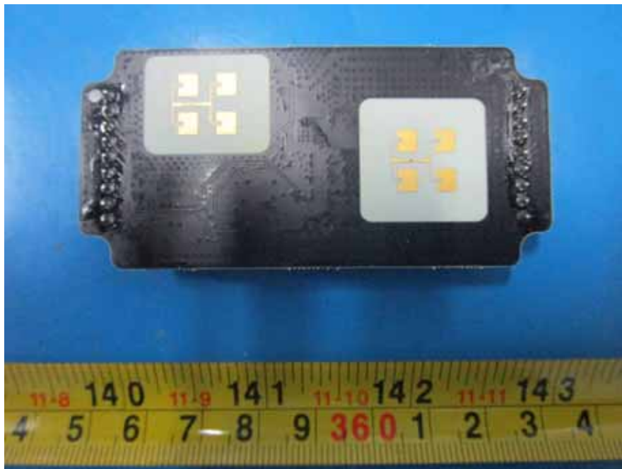
EUT –PCB Top And Antenna View
