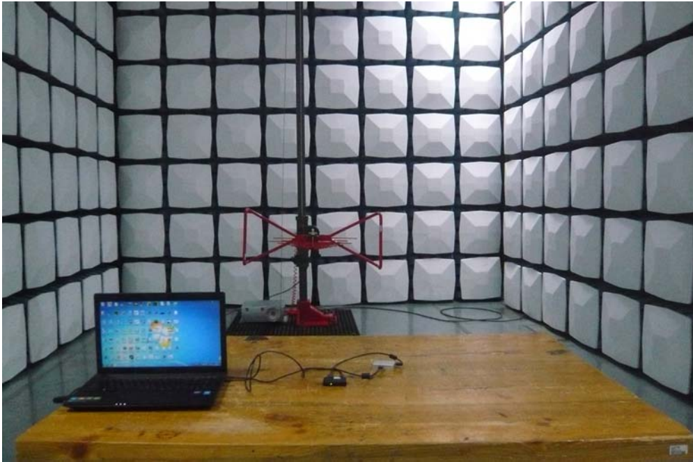
Radiated Emission View (Below 1GHz)-USB Mode
