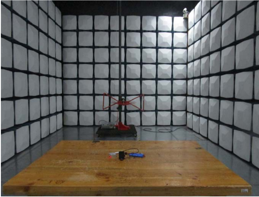
Radiated Emission View (Below 1GHz) -Battery Mode
