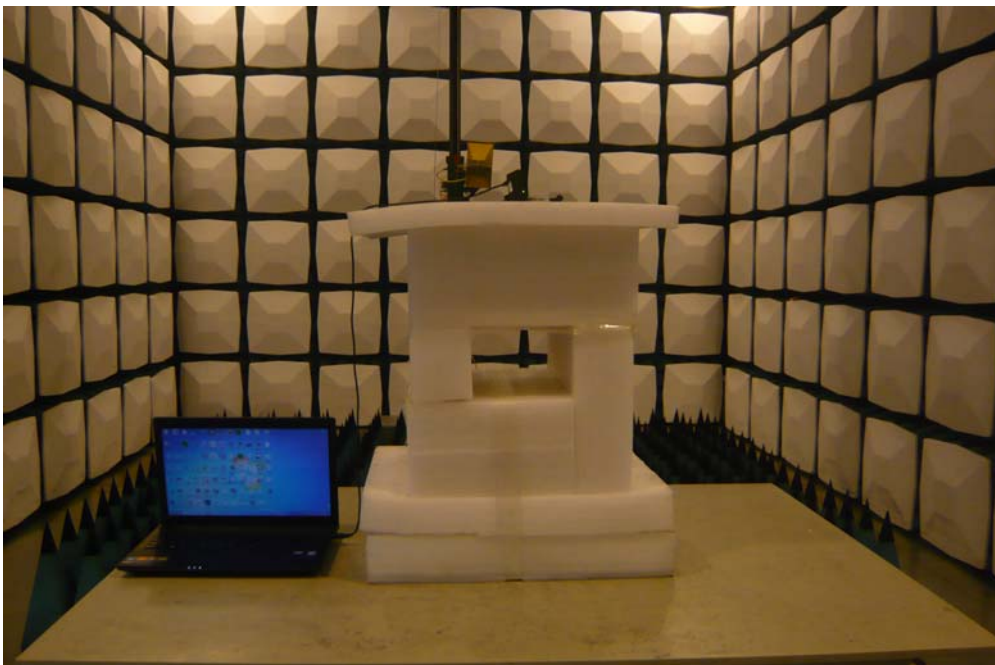
Radiated Emission View (Above 1GHz) -USB Mode
