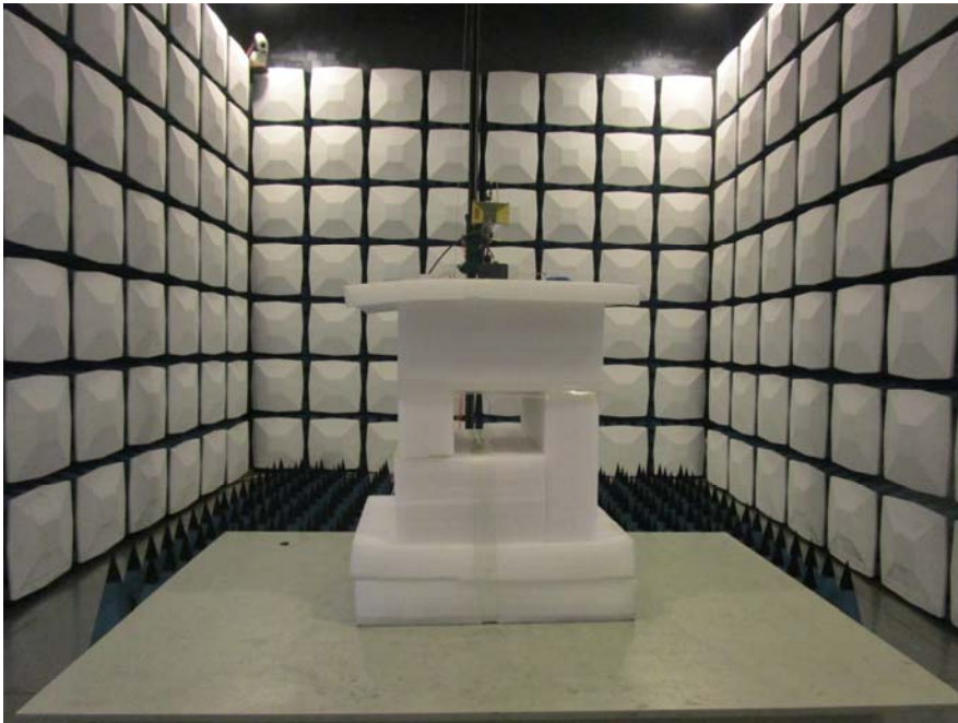
Radiated Emission View (Above 1GHz)-Battery Mode
