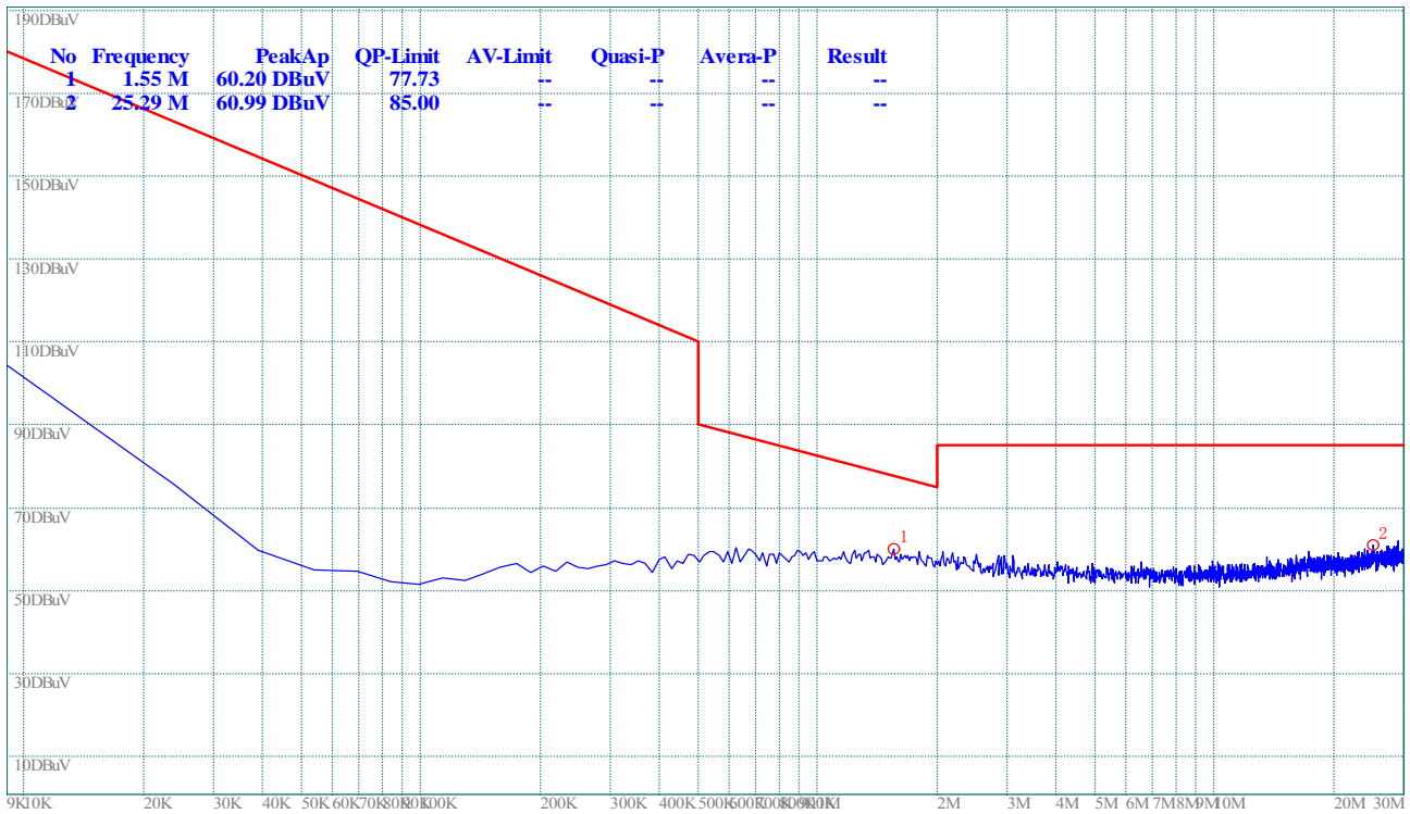
(Plot C.0: 9kHz to 30MHz, channel 36)
