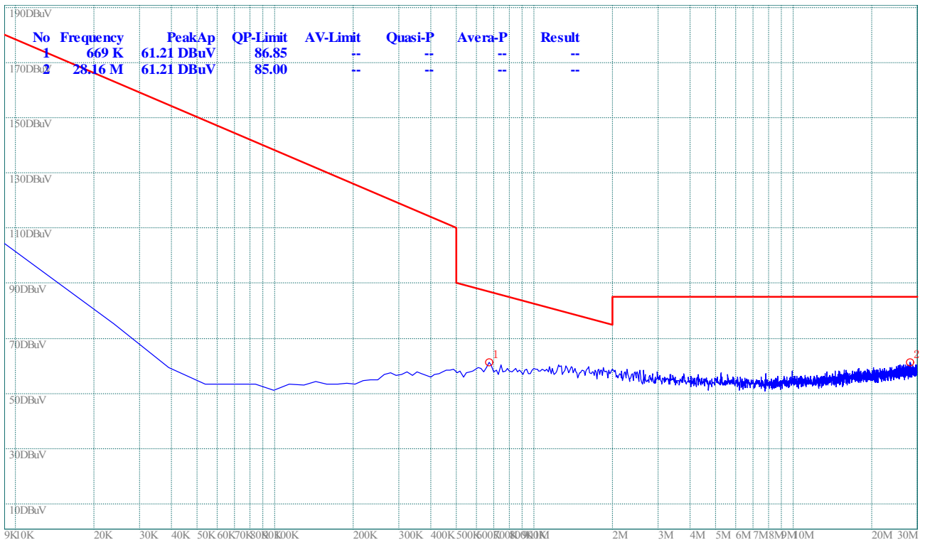
(Plot B.0: 9kHz to 30MHz, channel 18)
