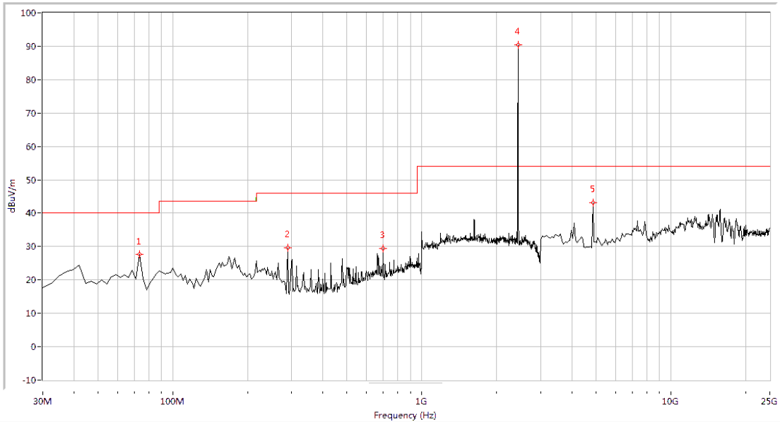
(Plot B.1: 30MHz to 25GHz, Antenna Horizontal, channel 18)
