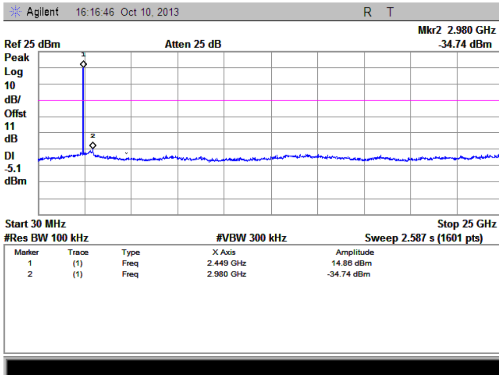
(Plot B.1: Channel = 18, 30MHz to 25GHz)
