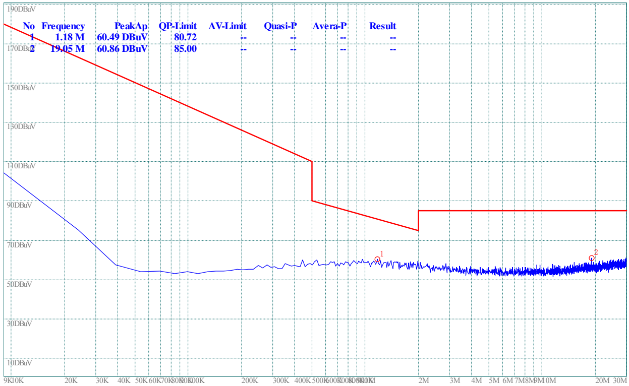
(Plot A.0: 9kHz to 30MHz, channel 1)
