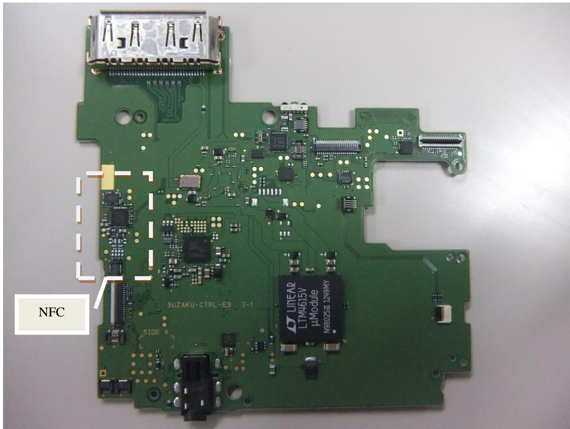
Photograph 1: Controller for SRX-SZKFULL (Front side)
