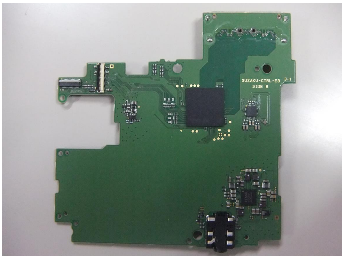
Photograph 2: Controller for SRX-SZKFULL (Back side)
