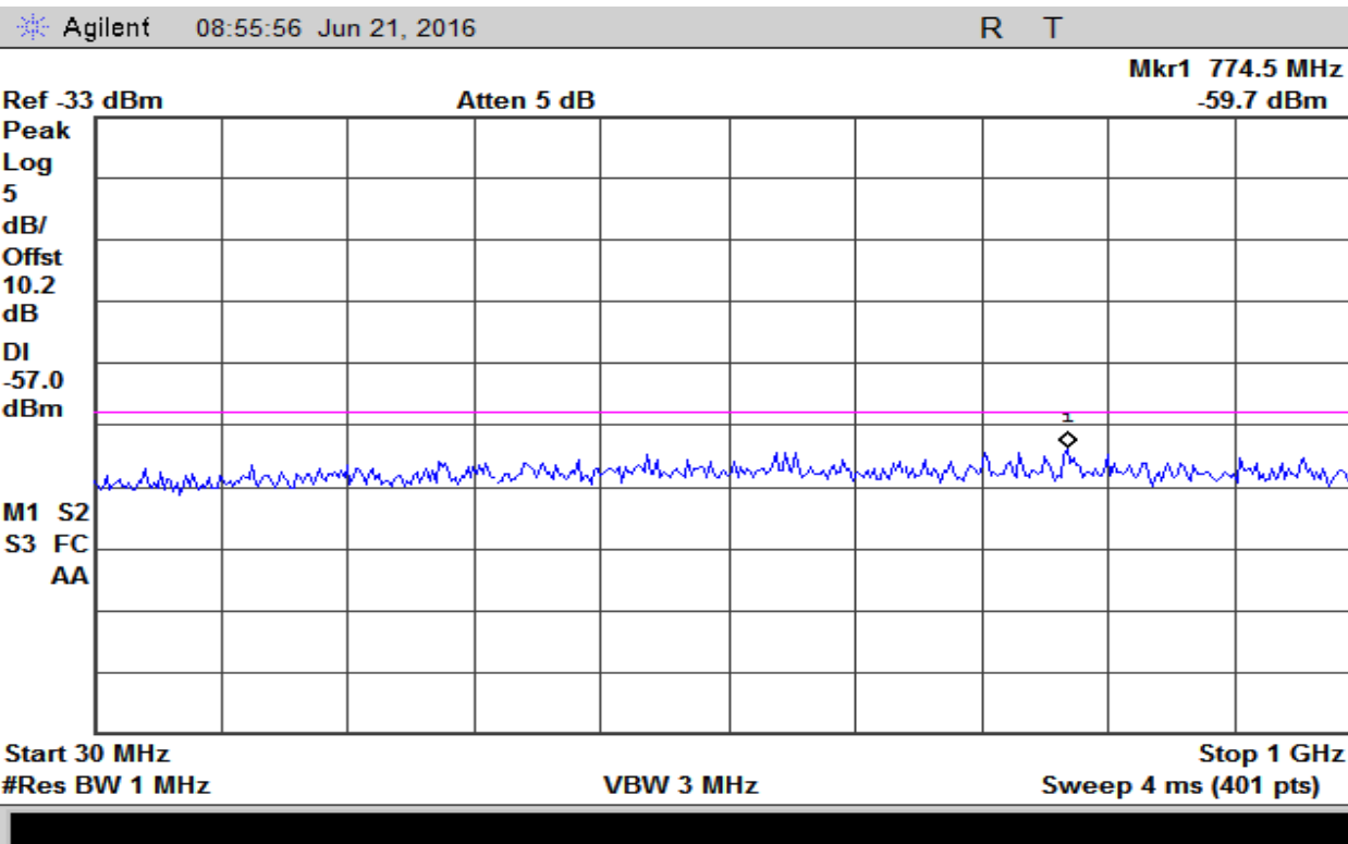
Plot 18 – Receiver Emission – For Industry Canada Only (RSS-GEN)
