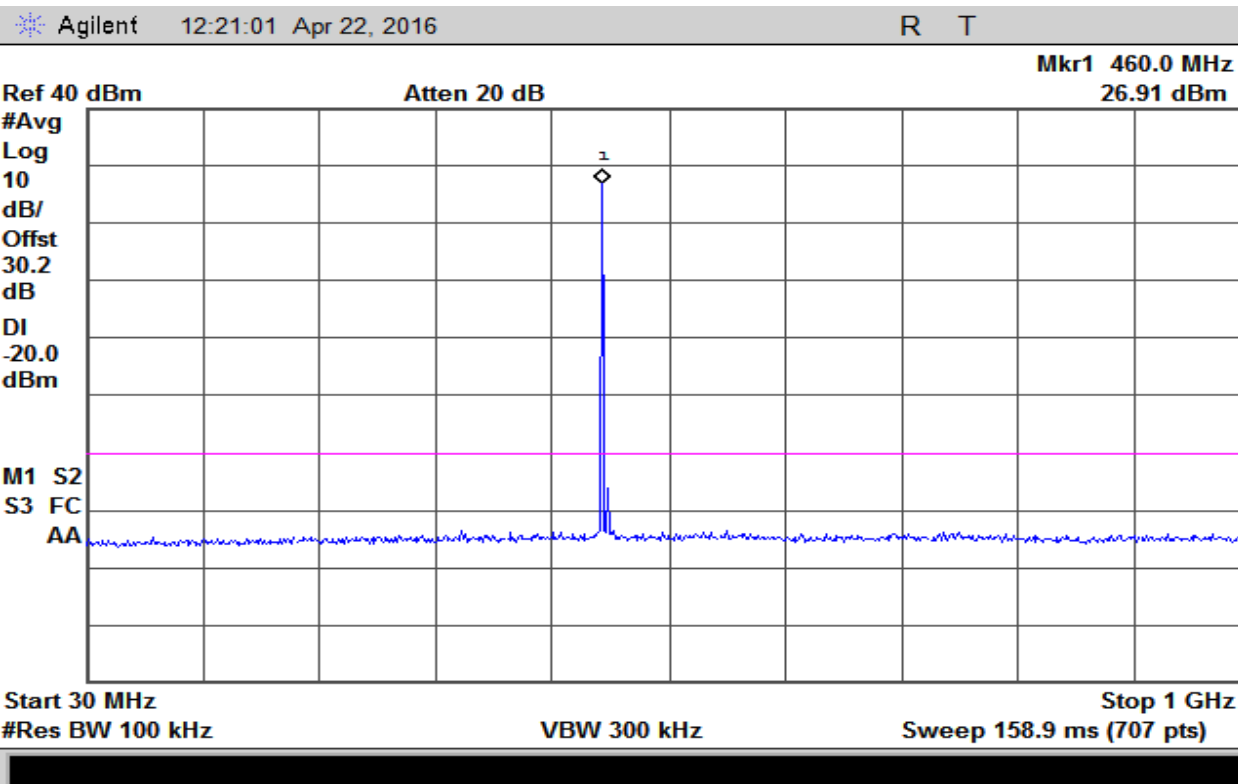
Plot 14 – Mid Band
