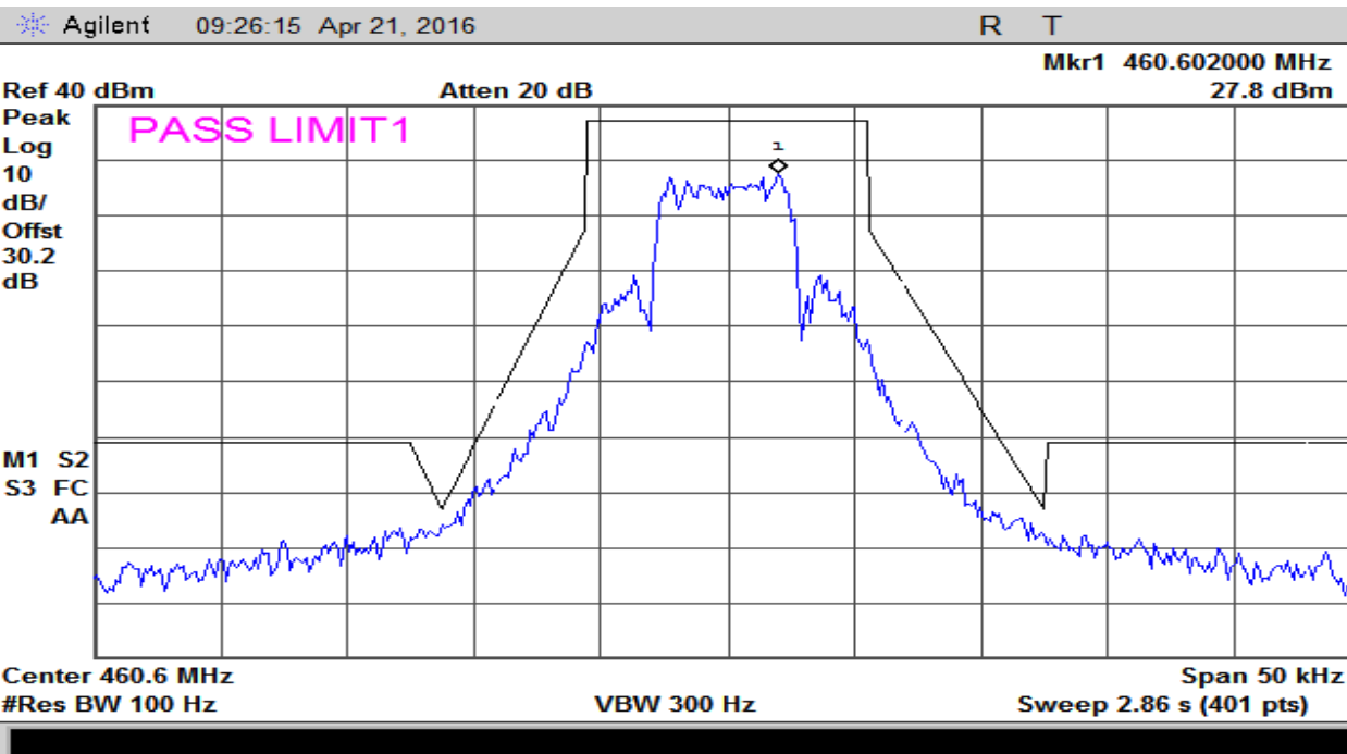
Plot 7 – Mid Chanel at Narrow Band 12.5 kHz Spacing – Mask D
