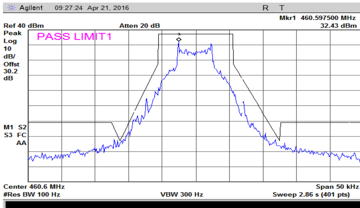
Plot 10 – Mid Chanel at Wideband Band 25 kHz Spacing – Mask D
