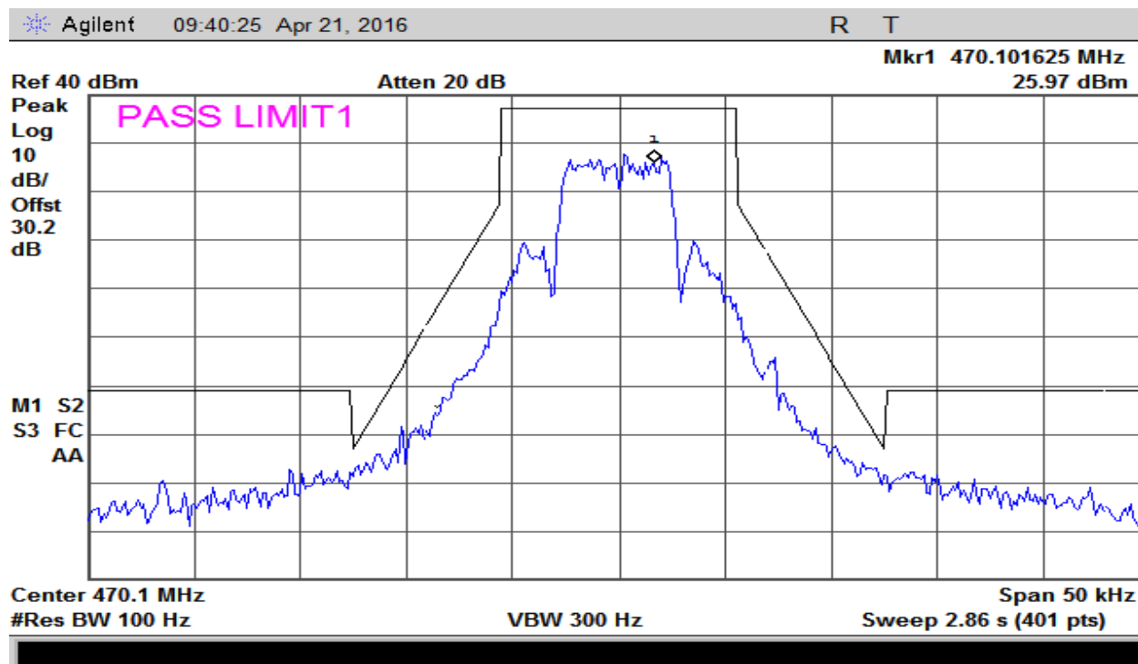
Plot 8 – High Chanel at Narrow Band 12.5 kHz Spacing – Mask D
