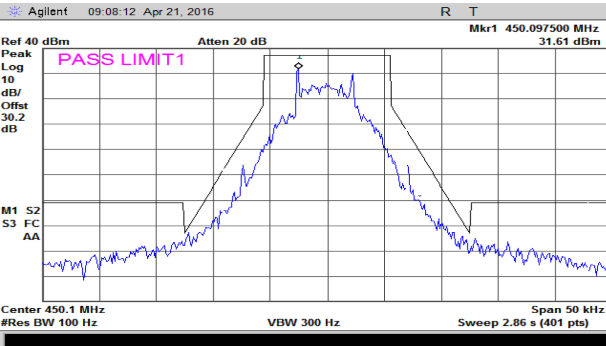
Plot 9 – Low Chanel at Wideband Band 25 kHz Spacing – Mask D
