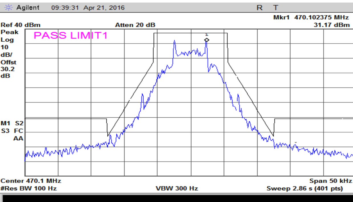
Plot 11 – High Chanel at Wideband Band 25 kHz Spacing – Mask D
