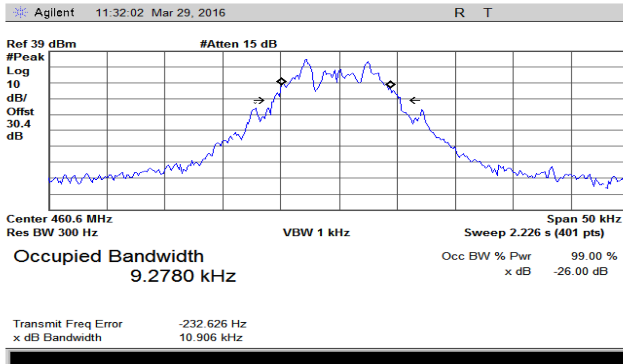
Plot 5 – Wide Band
